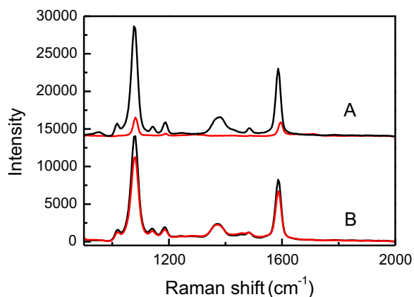
Fig. 4. SERS spectra of Ag@4-MBA (A) and Ag@4-MBA@SiO 2 (B) in water (black line) or whole blood (red line). Both spectra were obtained with 785 nm laser excitation. (For interpretation of the references to color in this figure legend, the reader is referred to the web version of this article.)
