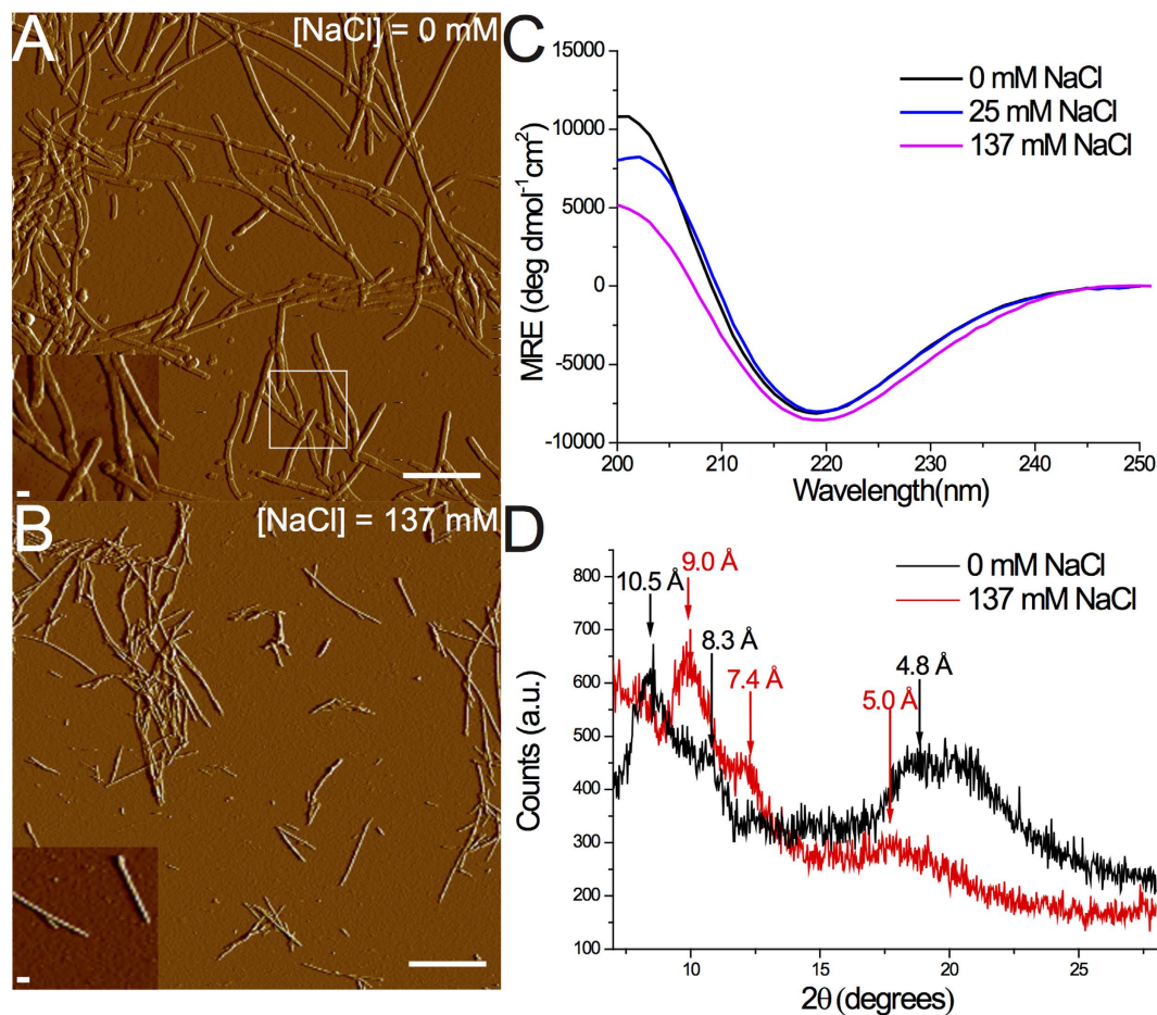
Figure 1. (A,B) AFM images (scale bar = 10 \mu m in main image and 100 nm in the inset), (C) UV-CD spectra, and (D) XRD spectra of \alpha S fibrils aggregated in the presence of varying concentrations of NaCl.
