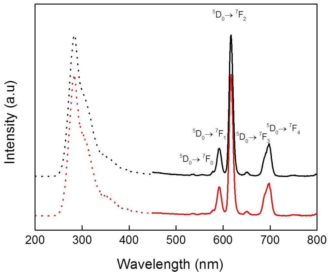
Figure S2. Excitation ( \lambda_{\text{em}} = 617 \text{ nm} , dotted line) and emission ( \lambda_{\text{ex}} = 280 \text{ nm} , continuous line) spectra of EuMo (red) and EuW (black) MOFs at room temperature.
