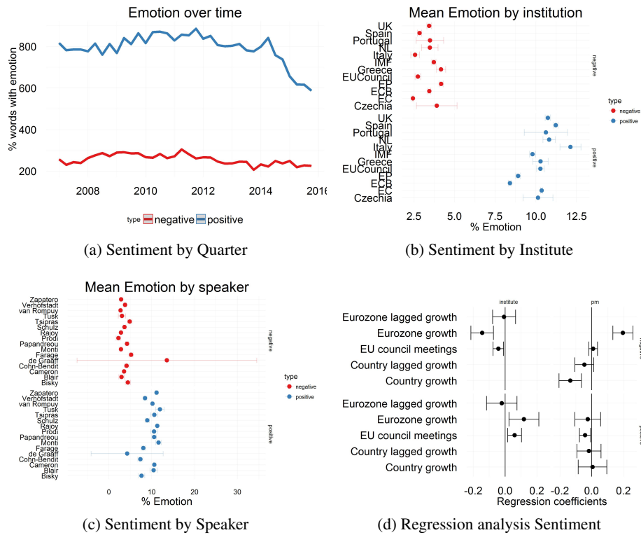
Figure 1: Sentiment Analysis
