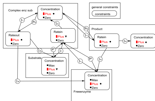
Figure 2. Causal dependencies compiled by Garp3 for state 4, providing a causal account for what is depicted by the value history graphs.
