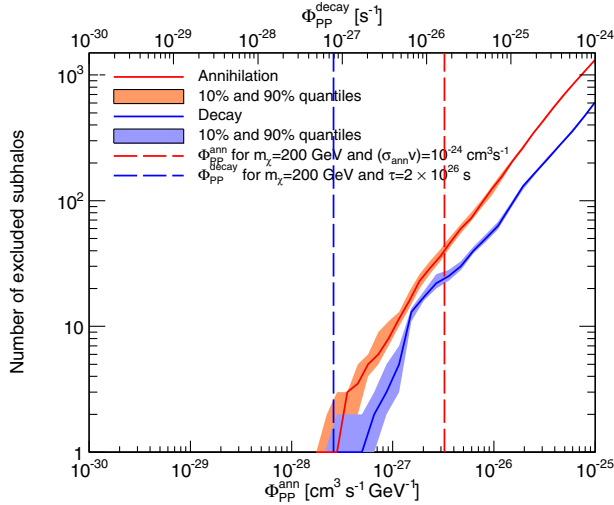
FIG. 21. The solid lines show the number of the DM subhalos in GAL-AQ with an energy flux above 0.1 GeV that is larger than 3 \times 10^{-12} erg cm ^{-2} s ^{-1} , i.e., the point-source sensitivity of Fermi LAT in the 3FGL catalog [92]. The solid lines denote the median over 100 independent realizations differing by the position of the observer and they are plotted as a function of the particle physics factor, in the case of an annihilating DM candidate (red line and bottom axis) and for a decaying one (blue line and top axis). In both cases, annihilations/decays into b\bar{b} are considered. The colored bands indicate the 10% and 90% quantiles among the 100 realizations. For reference, the \Phi_{\text{PP}}^{\text{ann}} for m_\chi = 200 GeV, \langle\sigma_{\text{ann}}v\rangle = 10^{-24} cm ^3 s ^{-1} and annihilation into b\bar{b} is marked by the dashed red line. Finally, the dashed blue line corresponds to the \Phi_{\text{PP}}^{\text{decay}} for m_\chi = 200 GeV, \tau = 2 \times 10^{26} s and decaying into b\bar{b} .
