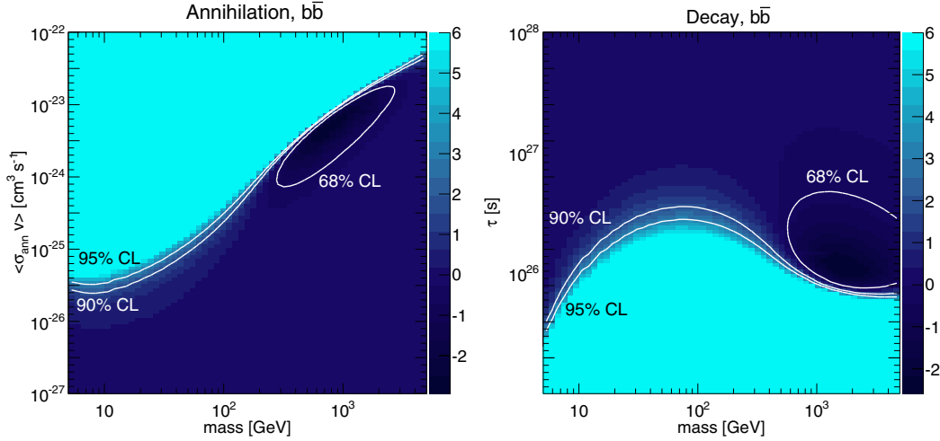
FIG. 27. \Delta\chi^2 between the best-fit solution for the two-component scenario and the best fit in the null hypothesis. Results presented here refer to the REF scenario for annihilation/decay into b\bar{b} and M_{\min} = 10^{-6} M_{\odot} . Left: Each point in the (m_{\chi}, \langle\sigma_{\text{ann}}v\rangle) parameter space is colored according to its \Delta\chi^2 , i.e. the difference between the \chi^2 of the best fit to the auto- and cross-APS in terms of the two-component model and the \chi^2 of the best fit of the null hypothesis (i.e. no DM). The closed white contour marks the 68% C.L. region. The 90% and 95% C.L. regions are below the white open curves labeled “90% C.L.” and “95% C.L.” respectively. Right: The same as the left panel but for decaying DM.
