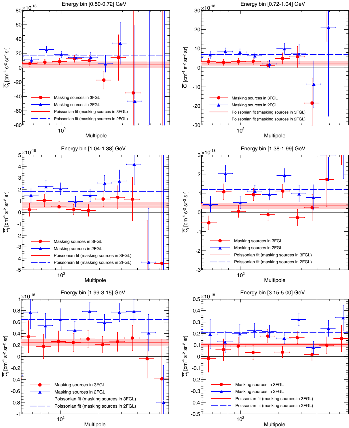
FIG. 29. Auto-APS of the IGRB for the first six energy bins and for the reference data set (P7REP_ULTRACLEAN_V15 front events) using the reference mask which excludes |b| < 30^\circ and 3FGL sources (red circles). The blue triangles show the same but masking the sources in 2FGL, instead. Data have been binned as described in Sec. IV A. The solid red line shows the best-fit C_P for the red data points, with the pink band indicating its 68% C.L. error. The dashed blue line corresponds to the best-fit C_P for the blue data points. The energy range is indicated on the top of each panel. Note that only the results in our signal region (i.e. between \ell = 49 and 706) are plotted and that the scale of the y-axis can vary from panel to panel.
