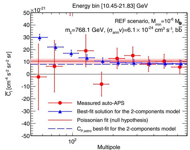
FIG. 26. Example of a fit to the binned APS \overline{C}_\ell in our particular energy bins, in terms of the two-component model described in the text. The red circles show the measured auto-APS in the energy bin between 10.4 and 21.8 GeV, as a function of the multipole. The solid red line is the Poissonian best-fit APS in the null hypothesis and the pink band denotes its estimated 68% C.L. error. The dashed blue line denotes the best fit of the Poissonian component when DM is included in the fit, for a DM mass of 768.1 GeV and a \langle\sigma_{\text{ann}}v\rangle of 6.12 \times 10^{-24} \text{ cm}^3 \text{ s}^{-1} , annihilation into b\bar{b} and a REF scenario with M_{\min} = 10^{-6} M_\odot . The best-fit signal (Poissonian plus DM component) is plotted by means of the blue triangles.
