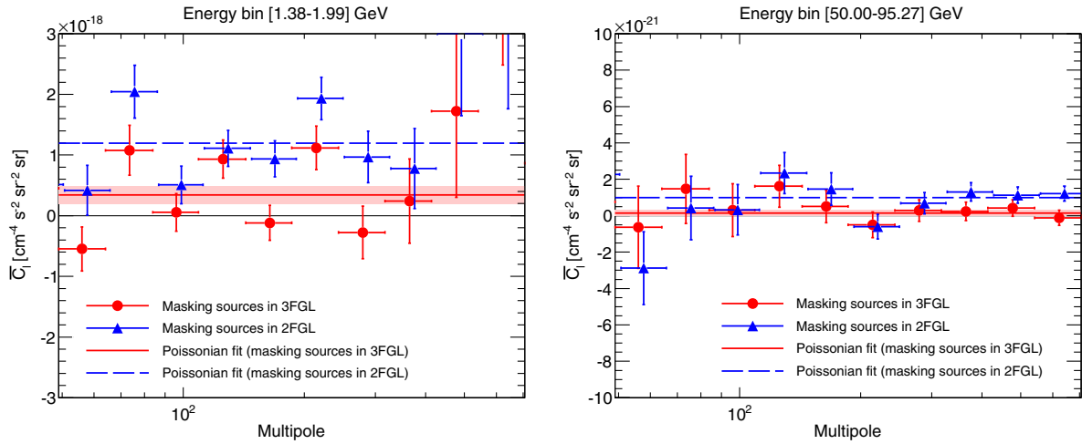
FIG. 6. Auto-APS of the IGRB for two representative energy bins (between 1.38 and 1.99 GeV in the left panel and between 50.0 and 95.27 GeV in the right panel) and for the reference data set (P7REP_ULTRACLEAN_V15 front events) using the reference mask which excludes |b| < 30^\circ and 3FGL sources (red circles). The blue triangles show the same but masking the sources in 2FGL. Data have been binned as described in Sec. IV A. The solid red line shows the best-fit C_P for the red data points, with the pink band indicating its 68% C.L. error. The dashed blue line corresponds to the best-fit C_P for the blue data points. Note that only the results in our signal region (i.e. between \ell = 49 and 706) are plotted and that the scale of the y-axis varies in the two panels. Also, the blue triangles have been slightly shifted horizontally with respect to the red circles to increase the readability of the plots. This will happen also in many of the following plots.
