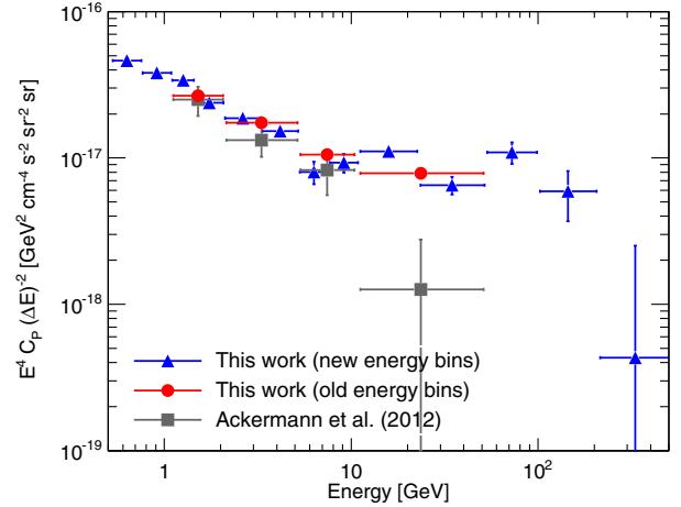
FIG. 18. Poissonian auto-APS as a function of energy for the default data set in this analysis, with 13 energy bins (blue triangles) and with the 4 energy bins used in Ref. [1] (red circles). Note that data are obtained using the mask that covers a 2^\circ circle around each source in 2FGL. The gray squares denote the measurement from Ref. [1] using the same mask.
