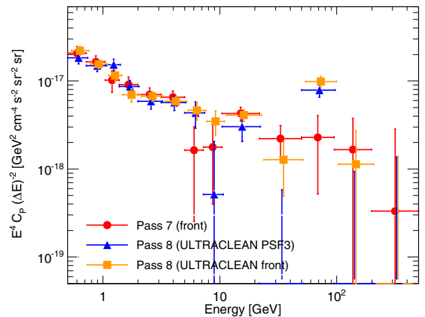
FIG. 15. Poissonian auto-APS as a function of energy for the Pass 7 (red circles), Pass 8 front (orange squares) and Pass 8 PSF3 (blue triangles) data sets. The default mask covering 3FGL sources is applied.
