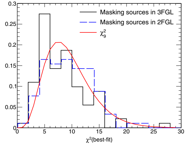
FIG. 10. Normalized distribution of the \chi^2 [defined as in Eq. (9)] for the best-fit Poissonian C_p for all 91 independent combinations of energy bins. The solid black line is for the case when 3FGL sources are masked and the dashed blue line is for the mask covering 2FGL sources. The solid red curve is a \chi^2 distribution with 9 degrees of freedom.
