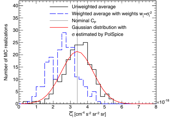
FIG. 4. Comparison between different methods to bin the auto-APS measured in the bin between \ell = 243 and 317 from the MC simulations described in the text. The nominal C_P is represented by the vertical gray line. The solid black histogram shows the distribution of the measured \overline{C}_\ell for the 200 simulated realizations, where the binned auto-APS is computed by an unweighted average. The dashed blue histogram denotes the case of a weighted average with weights given in Eq. (8). The solid red curve is a Gaussian distribution centered on the nominal C_P and with a standard deviation of 9.3 \times 10^{-19} \text{ cm}^{-4} \text{ s}^{-2} \text{ sr}^{-1} , as estimated with POLSPICE.
