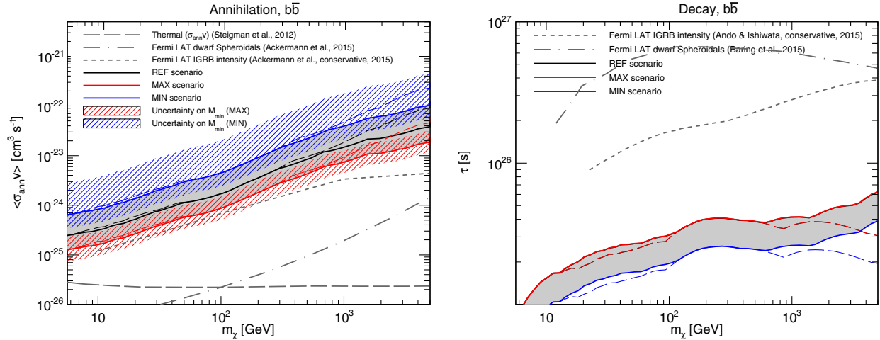
FIG. 25. Conservative exclusion limits on annihilating and decaying DM from the new APS measurement. Left: The solid lines show the upper limits on \langle\sigma_{\text{ann}}v\rangle derived from the auto- and cross-APS measured in Sec. III, as a function of m_\chi , for M_{\text{min}} = 10^{-6} M_\odot and annihilations into b\bar{b} . The limits follow the conservative approach described in the text. The black line is for the REF scenario, while the red and blue ones are for MAX and MIN, respectively. The gray band between the MIN and MAX scenario represents our estimated total astrophysical uncertainty for M_{\text{min}} = 10^{-6} M_\odot , accounting for all the sources of uncertainty mentioned in Sec. VII. The red and blue shaded bands describe the effect of changing M_{\text{min}} between 10^{-12} M_\odot and 1 M_\odot , for the MAX and MIN scenario. In the case of the black, red and blue dashed lines, the upper limits are derived only by considering the measured auto-APS and neglecting the cross-APS. For comparison, the long-dashed gray line marks the annihilation cross section for thermal relics from Ref. [94] and the dashed-dotted gray line the upper limit obtained in Ref. [95] from the combined analysis of 15 dwarf spheroidal galaxies. Finally, the short-dashed gray line shows the conservative upper limit derived in Ref. [31] from the intensity of the IGRB. Right: The same as in the left panel but for the lower limits on \tau for decaying DM. The short-dashed gray line represents the lower limit obtained in Fig. 6 of Ref. [96] from the IGRB intensity, while the dashed-dotted gray one is obtained from the combined analysis of 15 dwarf spheroidal galaxies in Ref. [97].
