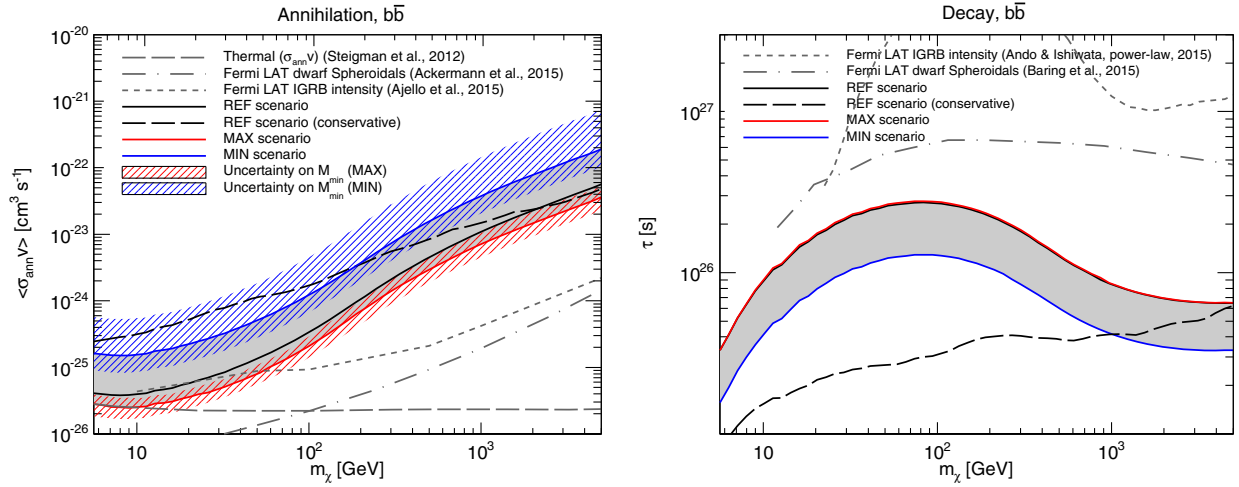
FIG. 28. Exclusion limits on annihilating and decaying DM from the fit to the binned \overline{C}_\ell in terms of the two-component model. Left: The solid lines show the upper limits that can be derived on \langle\sigma_{\text{ann}}v\rangle as a function of m_\chi (for annihilations into b\bar{b} quarks and M_{\text{min}} = 10^{-6} M_\odot ) by fitting the Fermi LAT data with a two-component model that includes astrophysical sources and DM (see text for details). The black, blue and red lines correspond to the REF, MIN and MAX scenario. The blue and red shaded areas indicate how the MIN and MAX upper limits change when leaving M_{\text{min}} free to vary between 10^{-12} M_\odot and 1 M_\odot . The black dashed line is the REF upper limit in the conservative case, from Fig. 25, while the long-dashed gray line is the thermal annihilation cross section from Ref. [94]. The dotted-dashed gray line is the upper limit derived in Ref. [95] from the combined analysis of 15 dwarf spheroidals, while the short-dashed gray line comes from the analysis of the IGRB intensity performed in Ref. [98]. Right: The same as in the left panel but for the lower limits on \tau , in the case of decaying DM. The short-dashed gray line represents the lower limit obtained in Ref. [96] from the IGRB intensity. The line is taken from Fig. 5 of Ref. [96], where the IGRB is interpreted in terms of a component with a power-law emission spectrum and a DM contribution. Finally, the dotted-dashed gray line is the upper limit from the analysis of 15 dwarf spheroidal galaxies performed in Ref. [97].
