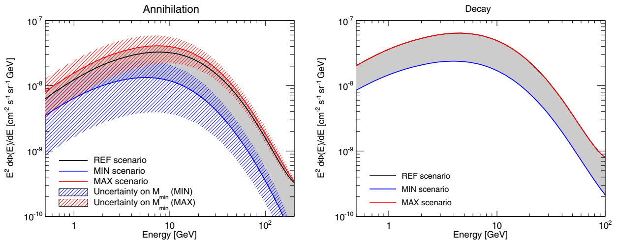
FIG. 23. Left: The predicted energy spectrum of the gamma-ray emission induced by the annihilation of a DM particle with a mass of 212 GeV, \langle\sigma_{\text{ann}}v\rangle = 3 \times 10^{-26} cm 3 s -1 and annihilation into b\bar{b} . The black line stands for the REF scenario, while the red and blue ones are for the MAX and MIN cases. Thus, the gray band determines the variability between the MIN and MAX scenarios. In all cases M_{\text{min}} = 10^{-6} M_\odot (see text for details). The red and blue shaded areas indicate how the MAX and MIN benchmarks change if we let M_{\text{min}} vary between 10^{-6} and 1 M_\odot . Right: The same as in the left panel but for a decaying DM particle with a mass of 212 GeV and a decaying lifetime of 2 \times 10^{27} s. The red and black lines overlap.
