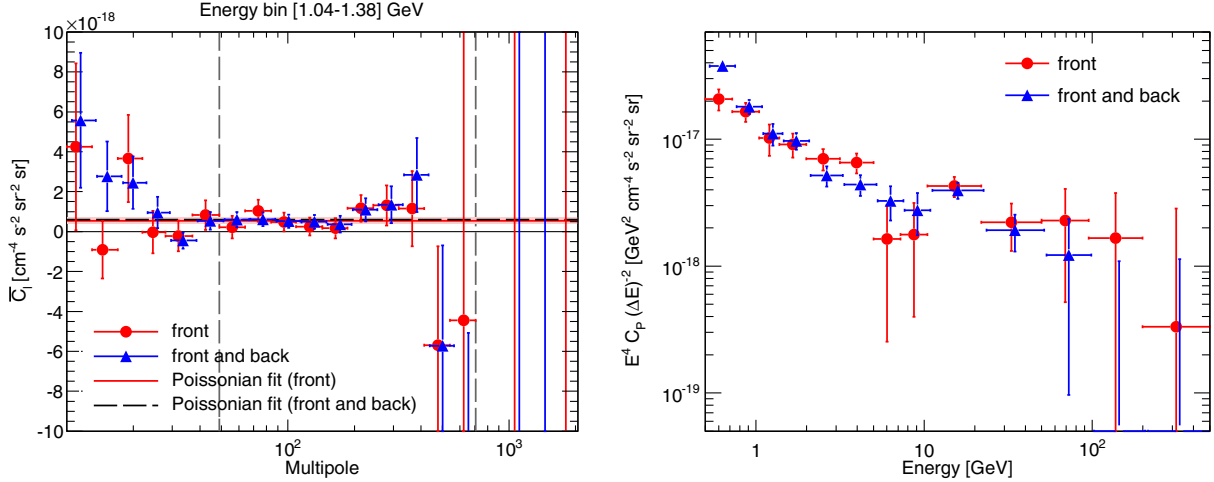
FIG. 16. Left: Comparison of the auto-APS in the energy bin between 1.04 and 1.38 GeV between the default data set which uses only front events (red circles) and the front + back data set (blue triangles). The solid red line marks the best-fit C_P for the default front-converting data, with the pink band indicating its 68% C.L. error. The dashed blue line gives the best-fit C_P for the front + back data set. The vertical gray dashed lines mark the signal region between \ell = 49 and 706. Right: Poissonian auto-APS as a function of energy for the front events (red circles) and the front + back ones (blue triangles). The default mask covering 3FGL sources is applied for both panels.
