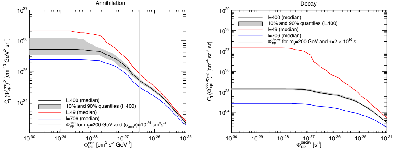
FIG. 22. Dependence of the APS of the GAL-AQ component on the particle physics factor defined in the text. Left: The solid lines show the DM-induced APS [computed above 0.1 GeV, for a fixed multipole and multiplied by (\Phi_{\text{PP}}^{\text{ann}})^{-2} ] as a function of \Phi_{\text{PP}}^{\text{ann}} , neglecting the DM subhalos that would be detected individually according to the Fermi LAT sensitivity threshold in the 3FGL catalog [92]. The black, red and blue lines are for \ell = 400 , \ell = 49 and \ell = 706 . They indicate the median over the 100 realizations with different positions for the observer, while the gray band (only for the case with \ell = 400 ) shows the variability between the 10% and 90% quantiles. For reference, the value of \Phi_{\text{PP}}^{\text{ann}} for m_\chi = 200 GeV, \langle\sigma_{\text{ann}}v\rangle = 10^{-24} cm 3 s -1 and annihilation into b\bar{b} is marked by the gray vertical line. Right: The same as in the left panel, but for a decaying DM candidate. The vertical gray line is the particle physics factor of a DM candidate with m_\chi = 200 GeV, \tau = 2 \times 10^{26} s and decaying into b\bar{b} . Note that the default mask covering 3FGL sources is employed when computing the auto-APS.
