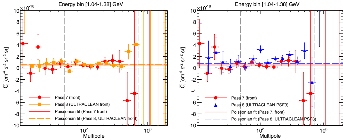
FIG. 14. Left: Comparison of the auto-APS measurement in the energy bin between 1.04 and 1.38 GeV between the default Pass 7 data set (red circles) and the Pass 8 front event selection (orange squares). Right: Same as the left panel but the comparison is between the Pass 7 data (red circles) and the Pass 8 PSF3 event selection (blue triangles). The solid red line marks the best-fit C_P for the default Pass 7 data set, with the pink band indicating its 68% C.L. error. The dashed orange (blue) line gives the best-fit C_P for Pass 8 front (PSF3) in the left (right) panel. The vertical gray dashed lines mark the signal region between \ell = 49 and 706. The default mask covering 3FGL sources is applied.
