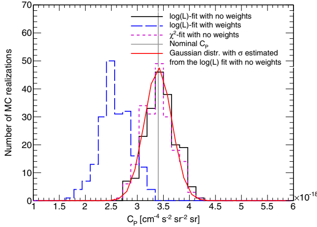
FIG. 5. Comparison between different methods to measure the Poissonian C_p in the MC simulations, given the binned \overline{C_\ell} . The nominal C_p is represented by the vertical gray line. The solid black histogram shows the distribution of the Poissonian C_p for the 200 simulated realizations obtained by maximizing the \log \mathcal{L} in Eq. (10) over the multipole range from 49 to 706. The binned \overline{C_\ell} 's in Eq. (10) are computed with no weights. If the weighted average is considered, the distribution of C_p is shown by the long-dashed blue histogram, which is clearly biased low. The short-dashed pink histogram shows the distribution of C_p computed by the minimization of the \chi^2 in Eq. (9) from \overline{C_\ell} binned with no weights. The solid red curve is a Gaussian distribution centered on the nominal C_p and with a standard deviation of 2.6 \times 10^{-19} \text{ cm}^{-4} \text{ s}^{-2} \text{ sr}^{-1} , as estimated from the \log \mathcal{L} method.
