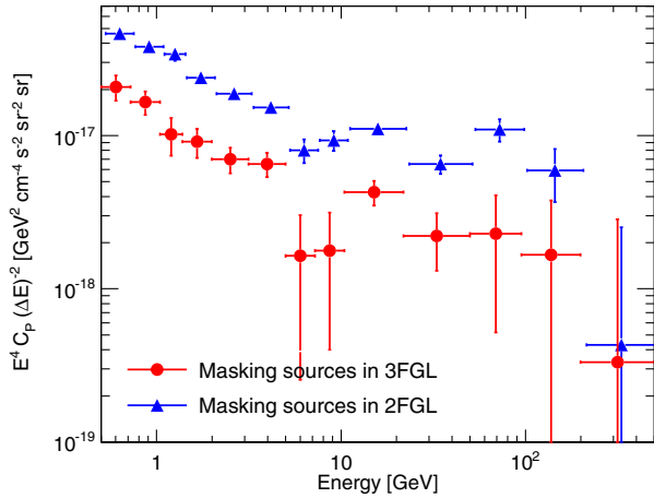
FIG. 8. Anisotropy energy spectra for the auto-APS using the reference data set with the default 3FGL mask (red circles) in comparison with the case in which we use the default mask around 2FGL sources (blue triangles).
