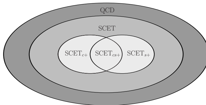
Figure 5. Schematic overview of the fixed-order content of the different theories discussed here. Approaching the cs+ regime in the center, more and more logarithms get large and are resummed, at the expense of additional expansions. The missing fixed-order corrections from these expansions can be incorporated by adding back the relevant nonlogarithmic fixed-order differences between the theories.
