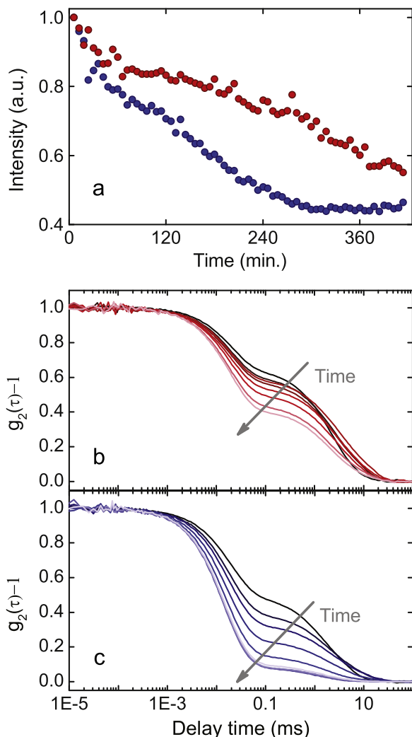
Fig. 5. Dynamic light scattering of quantum dot suspensions on the right side of the critical point. (a) Scattering intensity as a function of time at \Delta T=20^\circ\text{C} (●) and 1^\circ\text{C} (●). (b,c) Time evolution of the intensity correlation function at \Delta T=20^\circ\text{C} (b) and 1^\circ\text{C} . (c) Measurements were taken every hour (dark to light colour).
