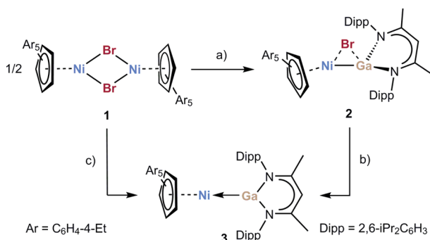
Scheme 1. Synthesis of Complexes 2 and 3 a
