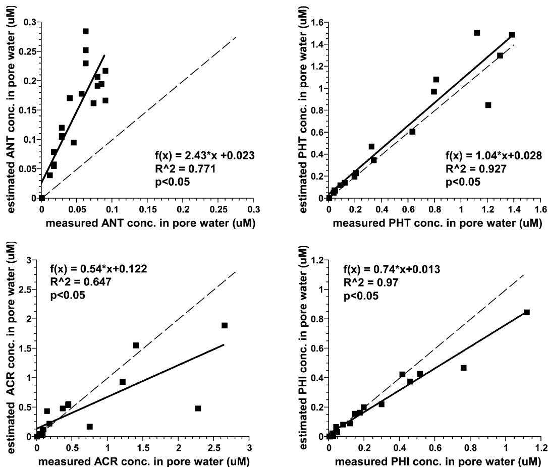
FIGURE 1. Relationship between polycyclic aromatic compound (PAC) concentrations in pore water estimated using SPME measurements (Y-axis, \mu\text{M} ) and measured experimentally (X-axis, \mu\text{M} ) in spiked Drontermeer sediment during 28-day toxicity tests with Lumbriculus variegatus . Dashed line represents 1:1 relationship.
