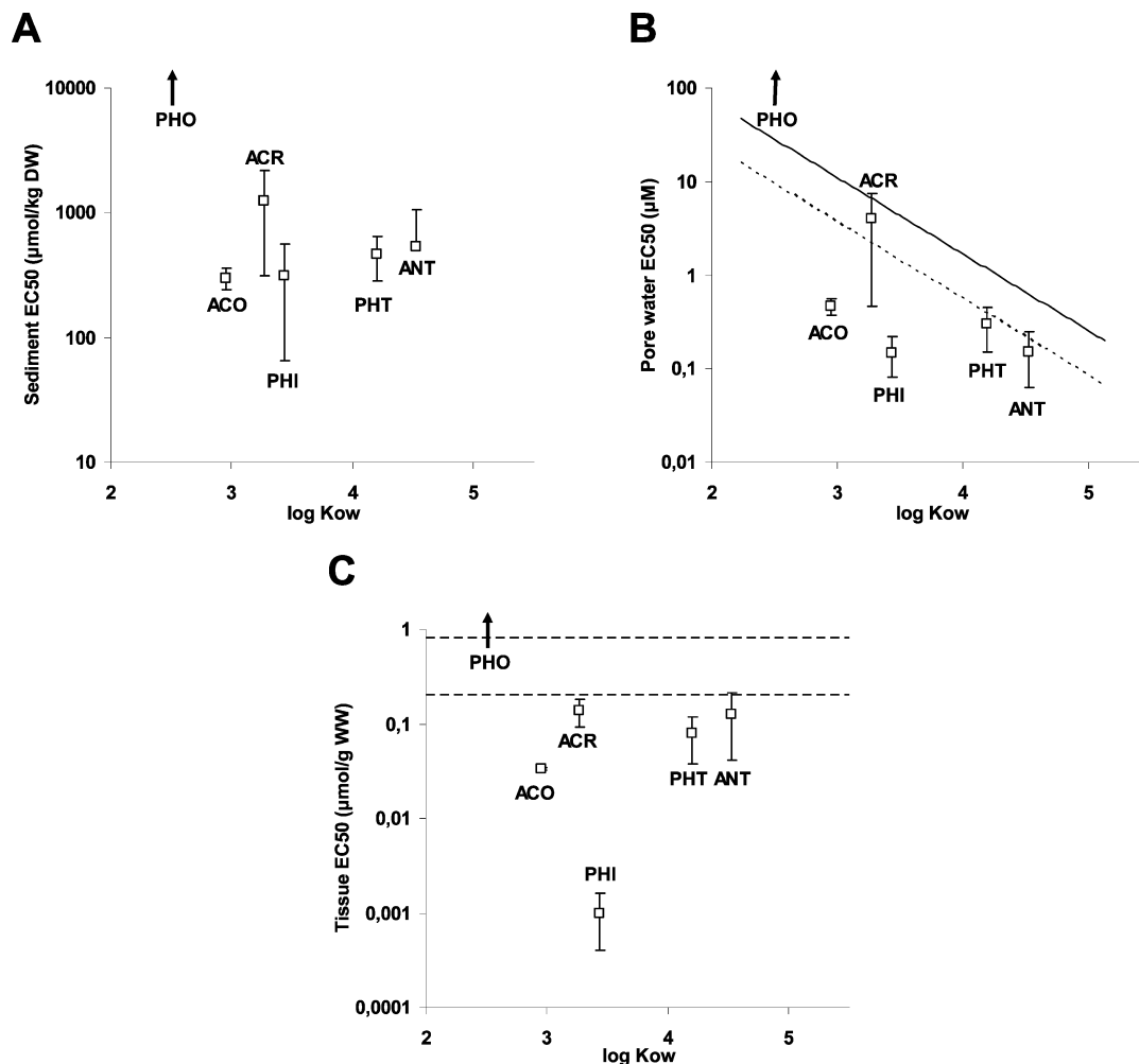
FIGURE 2. EC50 values for the effect of polycyclic aromatic compounds (PACs) on reproduction of Lumbriculus variegatus in spiked Drontemeer sediment as a function of log K_{ow} (•); based on measured concentrations in sediment ( \mu\text{mol}/\text{kg DW} , plot A), estimated concentrations in pore water ( \mu\text{M} , plot B) and concentrations in L. variegatus (ER50s, \mu\text{mol}/\text{g WW} , plot C). (Plot B) Solid line: linear log \text{LC}_{50} –log K_{ow} relationship for Chironomus riparius exposed for 96 h to similar PACs ( y = -0.8162x + 3.4936 , r^2 = 0.986 , (47)). Dashed line: ratio \text{LC}_{50} from ref (47)/3, lower limit for narcosis. For acridone, the calculated pore water EC50 is shown. (Plot C) Dashed lines: according to CBR predictions, upper and lower limits of the tissue concentration interval after chronic exposure to narcotic chemicals (0.2–0.8 \mu\text{mol}/\text{g WW} ).
