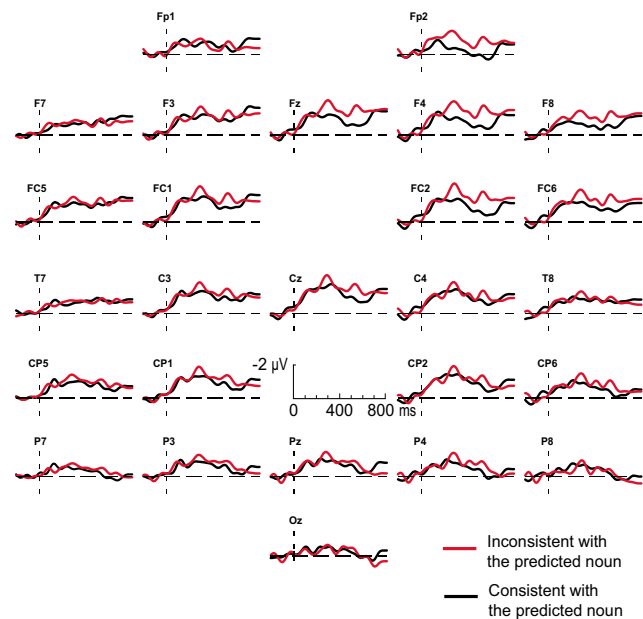
Figure 1 Adjectives in a predictive context. Grand average ERPs elicited by the critical adjectives in a predictive context. Black lines represent the response to adjectives bearing an inflection that is consistent with the gender of the predicted noun; red lines represent responses to gender inconsistent adjectives. The ERPs are timelocked to the onset of the adjective, and are filtered (8 Hz high cut-off, 48 dB/oct) for presentation purposes only. Note that in this and all following figures, negative polarity is plotted upward.
