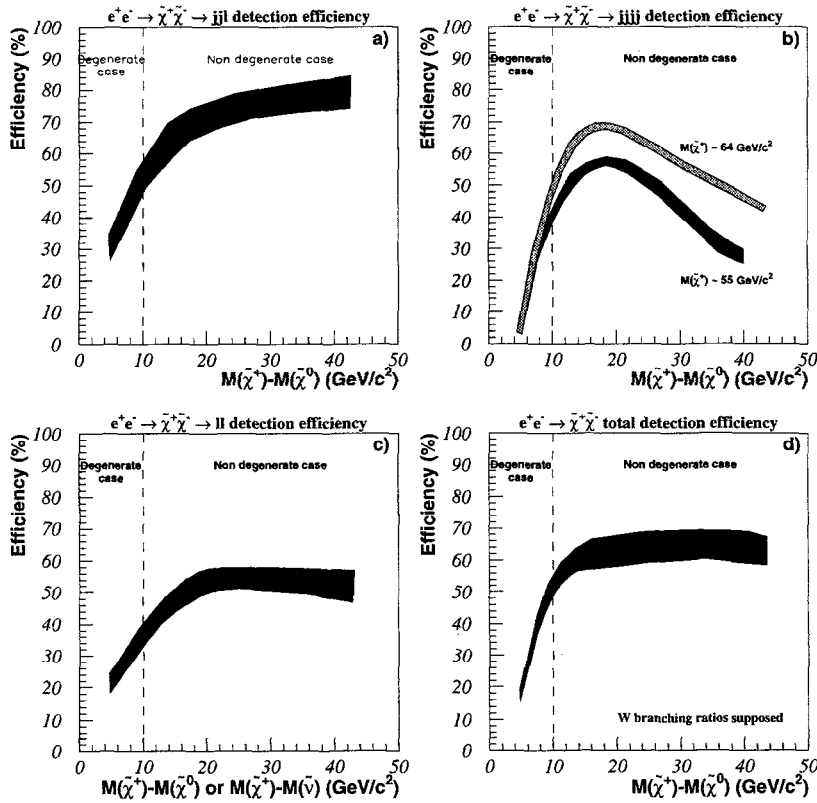
Fig. 1. Chargino detection efficiency for the three modes: a) JJ\ell , b) 4J and c) \ell\ell , obtained summing over the three selection criteria. d) Overall chargino detection efficiency obtained summing over the three selection criteria and assuming for the chargino decay branching ratios equal to those of the W . The bands correspond to the statistical error combined with the effect of generating points at different chargino masses.
