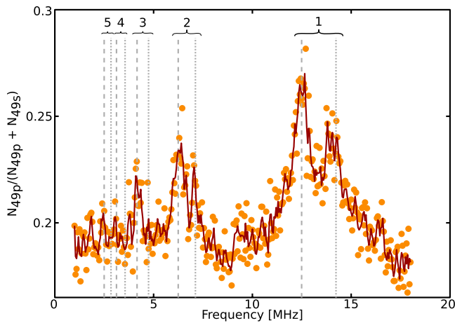
FIG. 7. (Color online) Observed frequency dependence of rf-assisted dipole-dipole transitions at F_S=0.26 V/cm. Multiphoton peaks with n=1-5 involved photons are clearly distinguishable; the number of involved photons is denoted in the figure. The double peak structure corresponds to the two resonances F_a and F_b . The solid line is a smooth spline fitted to the data.
