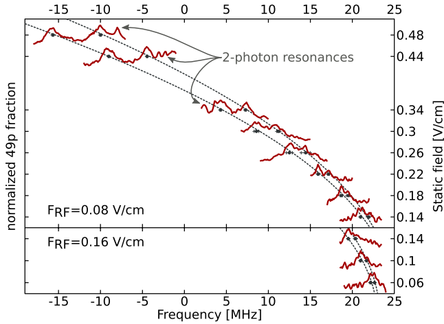
FIG. 9. (Color online) +1 and -1 photon resonances at various effective field values. In the lower panel (small static fields) the rf amplitude had to be increased leading to a larger ac Stark shift. The fitted resonance positions are marked by black dots. Some two-photon resonances are also visible and marked in the figure.
