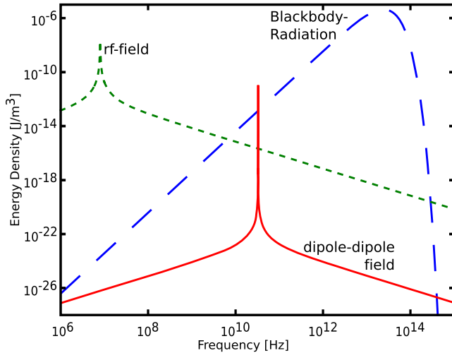
FIG. 2. (Color online) Energy density spectrum of the three different radiation fields, to which the atoms are exposed. The blue line (long dashes) represents the always and everywhere present blackbody radiation, depicted for 300 K. Resonances of the vacuum chamber and the metallic field plates are not taken into account for this illustration. The red line (solid) represents the photon that goes from one atom to the other, due to the dipole-dipole interaction at 25 \mu\text{m} . The line shape is Lorentzian based on experimental parameters. The green line (dashed) represents the oscillating field that is externally applied.
