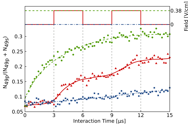
FIG. 6. (Color online) 49p fraction as a function of interaction time for different fields F=F_a (green circles), F=0 (blue squares), and F alternating between F_a and 0 in the manner depicted on top of the figure (red triangles). Lines depict a smooth spline fitted to the data.
