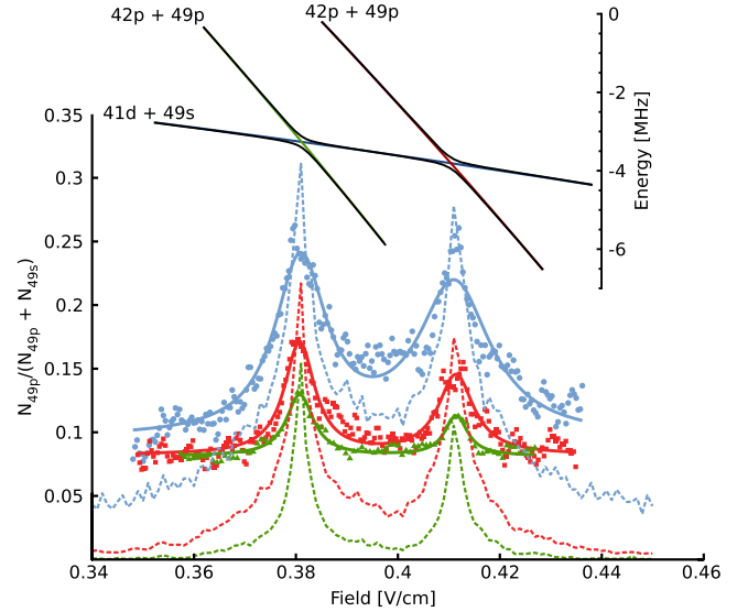
FIG. 5. (Color online) Static-field scans at 20- (blue circles), 30- (red squares), and 40- (green triangles) \mu m separation between the 41 d and the 49 s states. Solid lines are fits with two independent Lorentz profiles. Dashed lines are theoretical computations [7]. The inset shows the energy-level diagram for two atoms at 25 \mu m. The energy scale is relative to the energy of the 41 d +49 s state at zero field.
