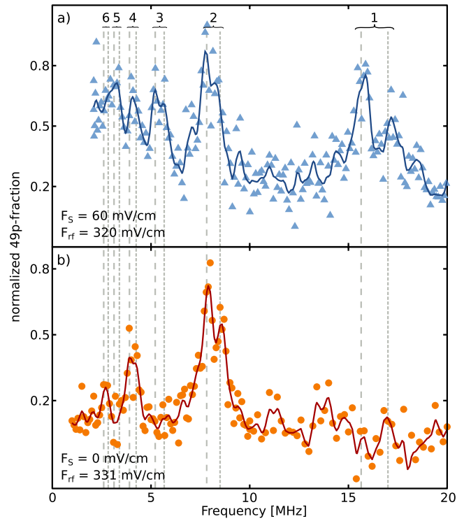
FIG. 8. (Color online) Measurements at small static field F_S (upper panel) and at F_S=0 (lower panel) showing selection rules prohibiting odd photon number transitions (see the text). The solid lines are a smooth spline fitted to the data.
