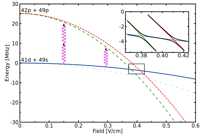
FIG. 3. (Color online) Schematic representation of two-atom energy versus electric field. An external rf field of 10 MHz is symbolized by the arrows. At a purely static field of 0.38 V/cm and 0.41 V/cm the dipole-dipole transition is resonant. At 0.3 V/cm it is brought into resonance by one rf photon of 10 MHz, while at 0.15 V/cm two such photons bring the system into resonance. The inset shows the avoided crossings due to dipole-dipole interaction at a separation of 25 \mu\text{m} .
