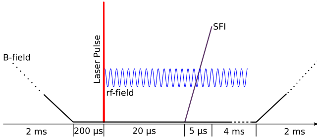
FIG. 4. (Color online) Schematic of the timing of one experimental cycle. First, the magnetic field is switched off, a laser pulse excites Rydberg states, which then are field ionized after 20- \mu s interaction time. Finally, the magnetic field is switched on again.
