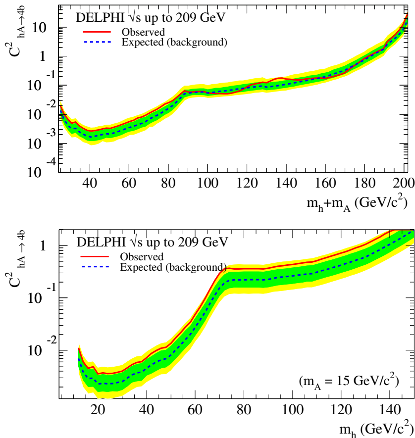
Fig. 14. 95% CL upper bounds on the reduction factor C_{hA \rightarrow 4b}^2 , as defined in Sect. 1.1. Results are presented for h and A bosons with equal masses (top) and with one mass fixed to 15 \text{ GeV}/c^2 (bottom). The limits observed in the data (full curve) are shown together with the expected median limits in background process experiments (dashed curve). The bands correspond to the 68.3% and 95.0% confidence intervals for background-only experiments
