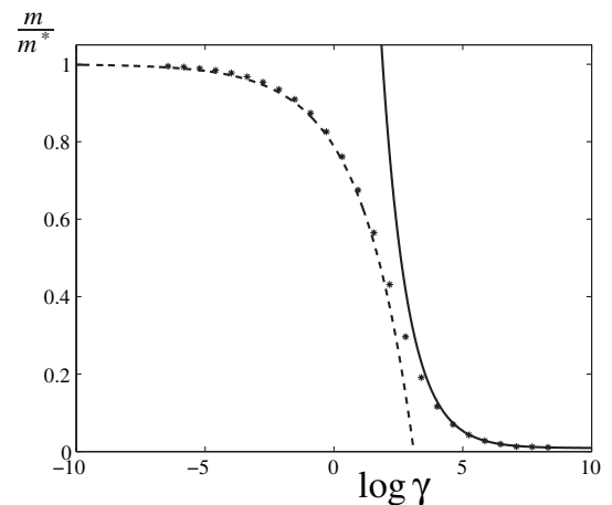
FIG. 1. Inverse effective mass m/m^* as a function of the dimensionless coupling constant \gamma (logarithmic scale). The stars (*) show numerical results for N = 111 particles, the solid curve represents the behavior in the strong coupling limit [Eq. (13)], and the dashed curve the behavior for a weak coupling [Eq. (18)].
