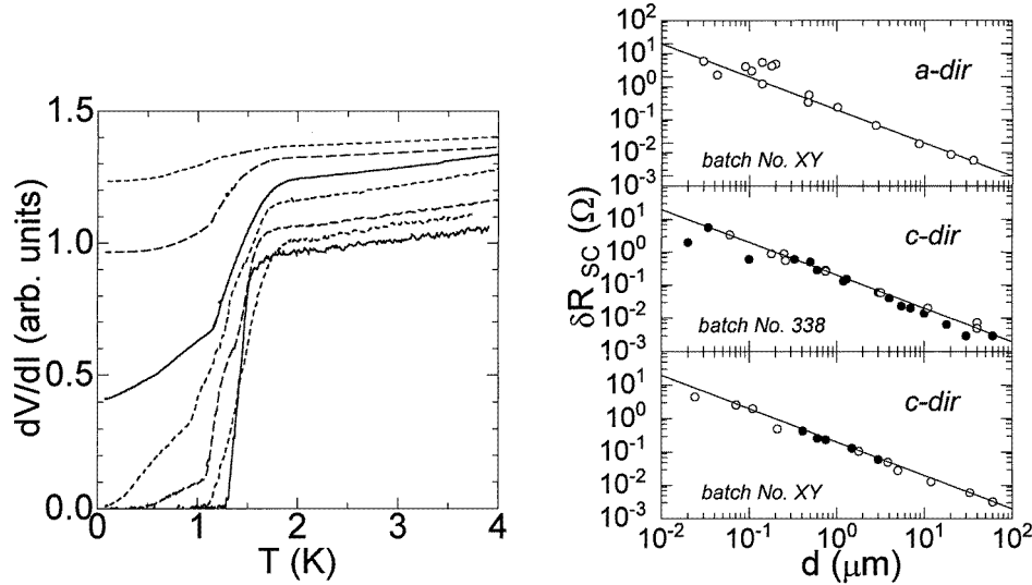
Figure 1. The differential contact resistance R = dV/dI at zero bias versus temperature T for \text{URu}_2\text{Si}_2 MCB along the c -direction. The resistance in the normal state at T \simeq 2 \text{ K} was (from top to bottom) 136, 10, 0.64, 1.4, 0.1, 0.03, and 0.003 \Omega , respectively.
