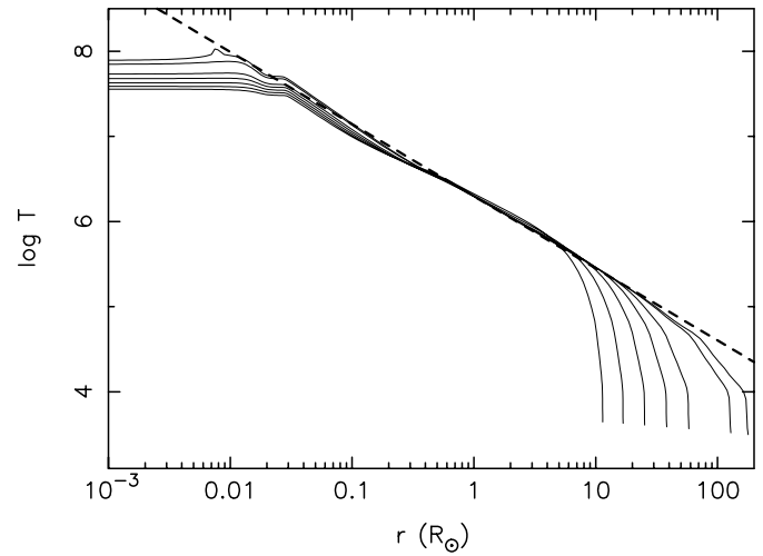
Fig. 1. The temperature profiles for 1 M_\odot evolved stars on the Red Giant Branch. Notice, that \log T is approximately a linear function of \log r at all evolutionary stages from the beginning until the tip of the Red Giant Branch (just before the helium flash).
