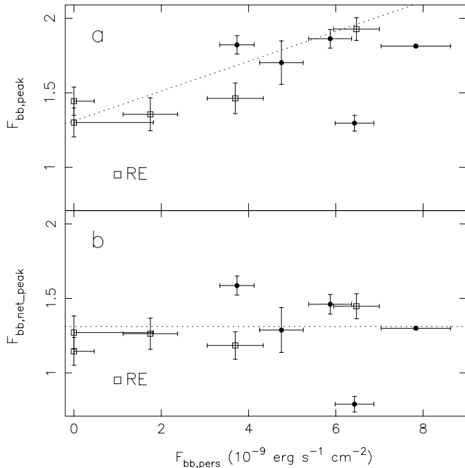
Fig. 10. a) Bolometric peak black-body flux (see text), F_{\text{bb,peak}} , in units of 10^{-8} \text{ erg s}^{-1} \text{ cm}^{-2} versus the bolometric persistent black-body flux, F_{\text{bb,pers}} . Radius expansion (RE) bursts are denoted with an open square. The dotted line represents a fit to the data points (excluding burst b2 and b3) to the function F_{\text{bb,peak}} = F_{\text{bb,pers}} + C . The constant C corresponds to (1.31 \pm 0.03) \times 10^{-8} \text{ erg s}^{-1} \text{ cm}^{-2} . b) Bolometric peak black body flux from spectral fits after subtraction of the persistent emission (see text), F_{\text{bb,net\_peak}} , in units of 10^{-8} \text{ erg s}^{-1} \text{ cm}^{-2} versus F_{\text{bb,pers}} . Radius expansion (RE) bursts are denoted with an open square. The dotted line represents the constant C .
