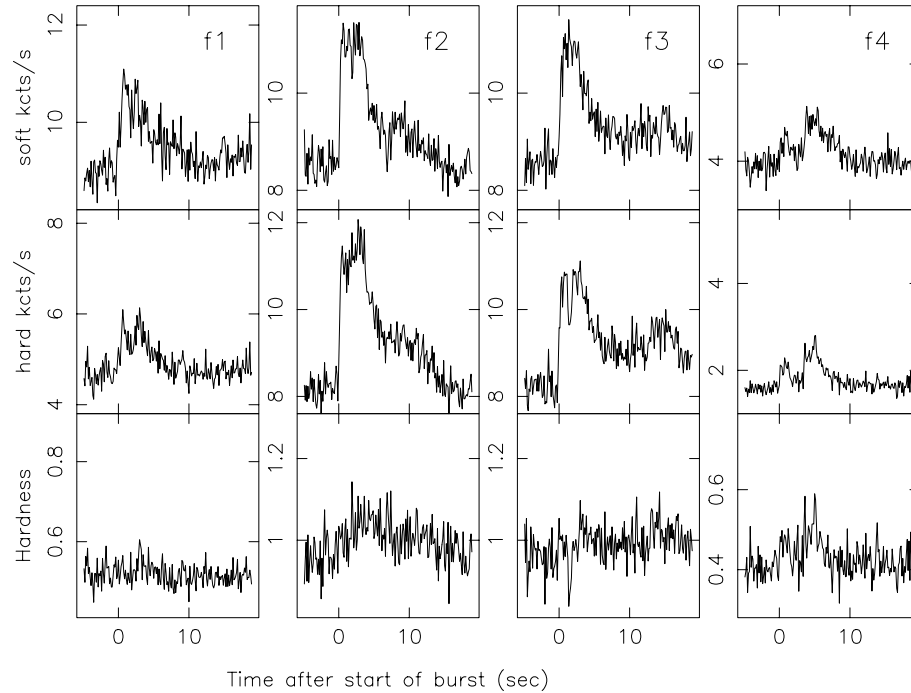
Fig. 2. The X-ray flare light curves at low (upper panels) and high (middle panels) energies and the corresponding hardness curves (lower panels), all at a time resolution of 0.125 s, for the four flares (f1–f4; see text). Time zero is the flare start time as given in Table 2. The low and high energy ranges are 1.5–7.2 keV and 7.2–19.7 keV, respectively, for f1, 1.9–6.2 keV and 6.2–19.6 keV, respectively, for f2 and f3, and 2.1–7.1 keV and 7.1–19.9 keV, respectively, for 4. Hardness is defined as the count rate ratio of the high to low energy band. No corrections for background and dead-time have been applied.
