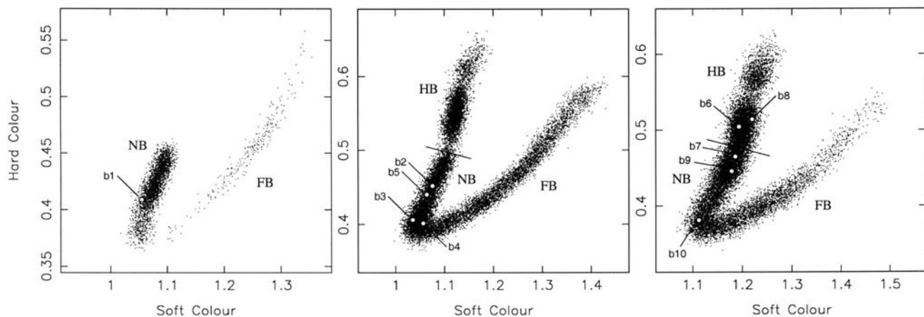
Fig. 16. Colour-colour diagrams of the RXTE/PCA observations of GX 17+2 (after Homan et al. 2001). The left, middle and right panels refer to the observations done during RXTE gain epochs 1, 3 and 4, respectively. The soft colour is defined as the count rate ratio in the 4.8–7.2 keV to the 3.0–4.8 keV energy bands for the epoch 1 data, in the 4.8–7.3 keV to the 3.0–4.8 keV energy bands for the epoch 3 data, and in the 4.6–7.1 keV to the 3.0–4.6 keV energy bands for the epoch 4 data. The hard colour is defined as the count rate ratio in the 10.6–19.7 keV to the 7.2–10.6 keV energy bands for the epoch 1 data, in the 10.5–19.6 keV to the 7.3–10.5 keV energy bands for the epoch 3 data, and in the 10.5–19.5 keV to the 7.1–10.5 keV energy bands for the epoch 4 data. Each point represents an average of 16 s. We have indicated the position of the source during 64 s intervals just before a burst (indicated by b1, b2, ..., b10, in chronological order), and the three limbs of the Z (HB, NB, FB). Since the HB is not clearly distinguishable from the NB in this figure, we have indicated the approximate HB/NB vertex by a line.
