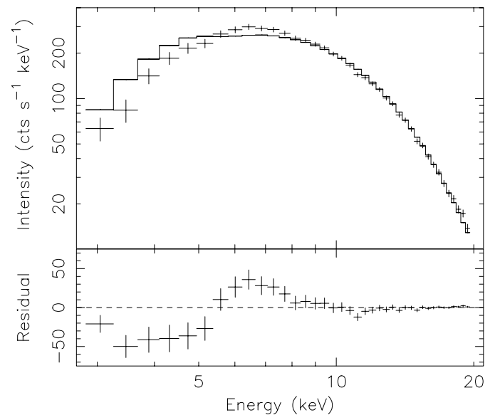
Fig. 14. Top panel: average observed net burst (i.e. total source minus persistent emission) spectrum during the flat top of burst b6, i.e. from 27 to 187 s after the start of the burst. A black-body fit is shown ( kT_{\text{bb}} = 2.658 \pm 0.015 \text{ keV} , R_{\text{bb},10} = 4.65 \pm 0.06 \text{ km} , \chi^2_{\text{red}} = 2.4 for 37 d.o.f.). Bottom panel: residuals after subtracting the best fit black-body model from the observed spectrum.
