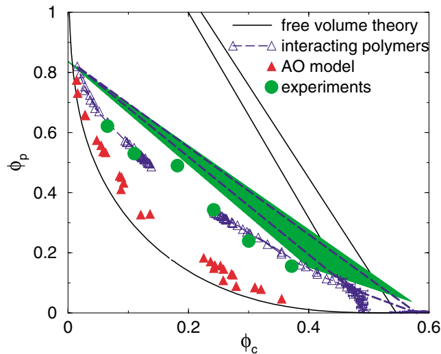
FIG. 2 (color online). Phase diagram in the polymer volume fraction-colloid volume fraction representation for q = 0.67 . Symbols as in Fig. 1. The large triangular areas denote the estimates for the triple point: the shaded area corresponds to the experimental data [3]. The simulated binodal agrees quantitatively with the experimental data of Ref. [7].
