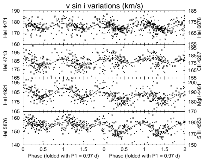
Fig. 9. Apparent v \sin i (in \text{km s}^{-1} ) for each line folded in phase with frequency f_1 = 1.03 \text{ c d}^{-1} . A best sinusoidal fit is overlaid.
