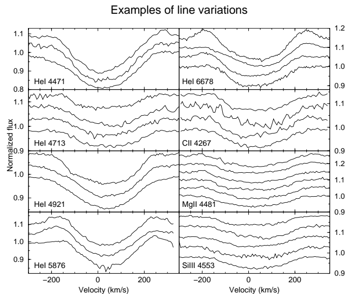
Fig. 3. Examples of typical variations for each studied line. The different normalized profiles have been vertically shifted by 0.05 to facilitate comparison.
