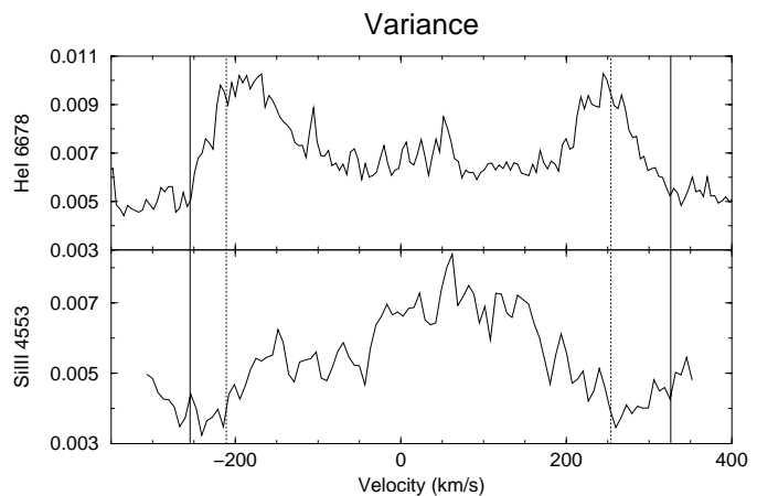
Fig. 4. Variance of the He I 6678 and Si III 4553 lines. The limits of the He I 6678 line are indicated as solid lines and of the Si III 4553 line as dotted lines, on both panels.
