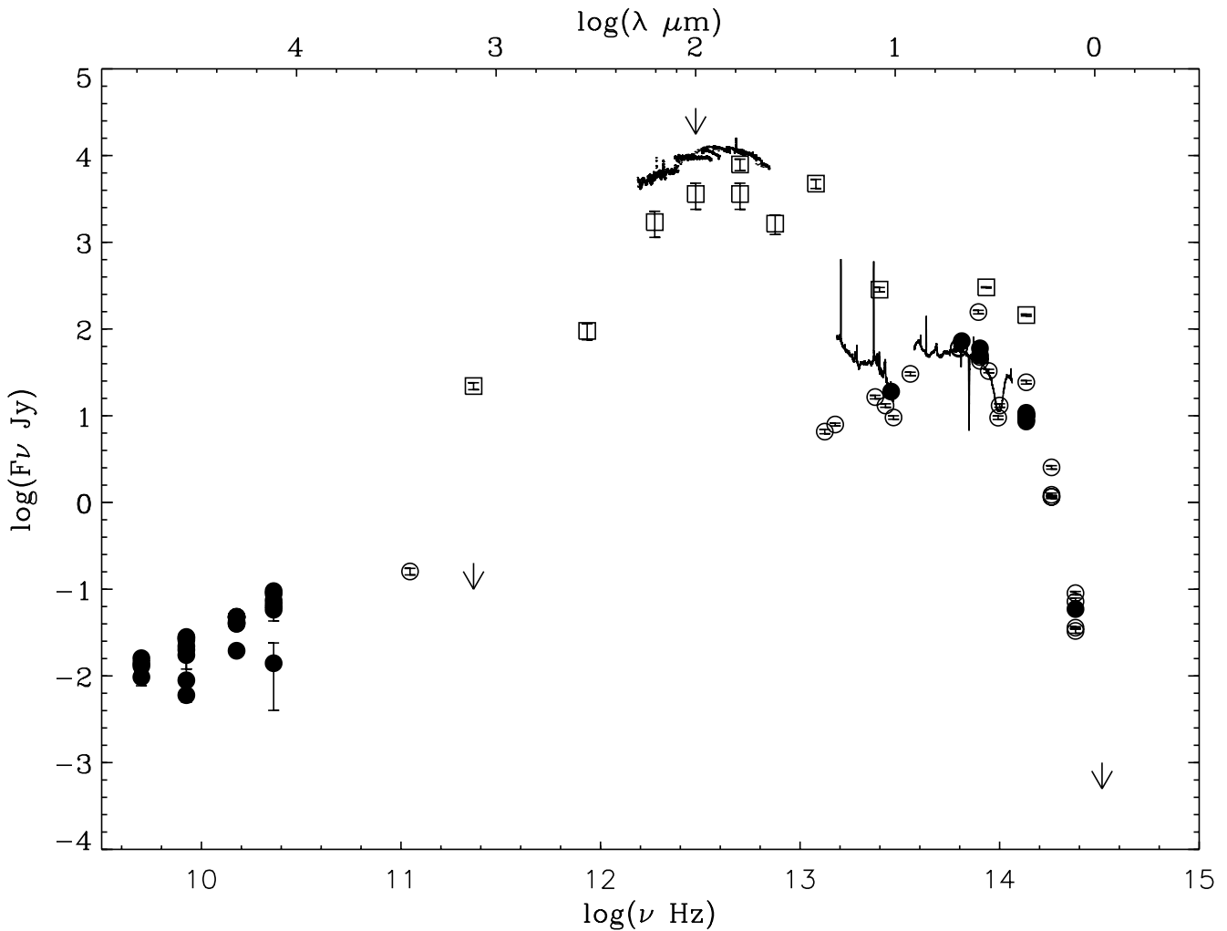
Fig. 4. The spectral energy distribution of IRS2, compiled from published photometric data and ISO SWS/LWS spectra. Details concerning these data are given in Tables 2–4. The high resolution ISO spectra (shown as continuous lines) are obtained in AOT6 mode. Open squares denote measurements made with apertures larger than 40'' ; open circles indicate aperture sizes of 5\text{--}20'' ; closed circles represent beam sizes less than 5'' . Most often, the error bars on the data are smaller than the symbol size. The subdivision in aperture size clearly shows that the emission bump peaking at about 100\ \mu\text{m} is not due to the nearby circumstellar medium of IRS2, i.e. it is not associated with the system itself but must come from warm material in the vicinity of the star.
