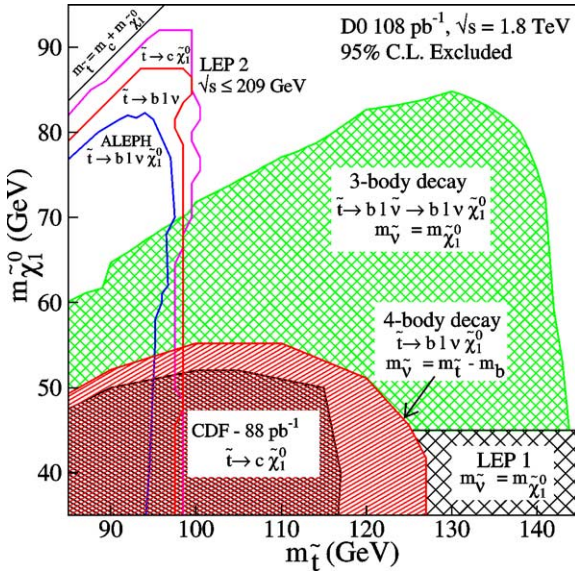
Fig. 4. Excluded regions in the (m_{\tilde{t}}, m_{\tilde{\chi}_1^0}) plane for the \tilde{t} \rightarrow b\ell\nu\tilde{\chi}_1^0 decay channel in the MSSM, assuming 3- or 4-body decay with a light sneutrino mass equal, respectively, to m_{\tilde{\chi}_1^0} and m_{\tilde{t}} - m_b . The chargino mass is assumed to be m_{\tilde{\chi}_1^\pm} = 140 GeV. The 3-body decay result was established in Ref. [6] and is compared to the LEP 1 (invisible width) and LEP 2 ( \tilde{t} \rightarrow b\ell\nu ) results under the same assumption ( m_{\tilde{\nu}} = m_{\tilde{\chi}_1^0} ). The results of this analysis are also compared to the exclusion limits obtained for the \tilde{t} \rightarrow c\tilde{\chi}_1^0 decay channels at LEP 2 and at the Tevatron by the CDF collaboration, and for the \tilde{t} \rightarrow b\ell\nu\tilde{\chi}_1^0 decay channel at LEP 2 by the ALEPH collaboration.
