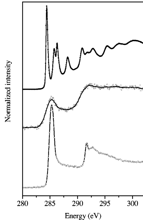
FIG. 2. C 1s core excitation spectra of concentric-shell fullerenes ( \circ ), graphite (momentum transfer parallel to the (001) direction ( \diamond ), and C_{60} ( \bullet ).
