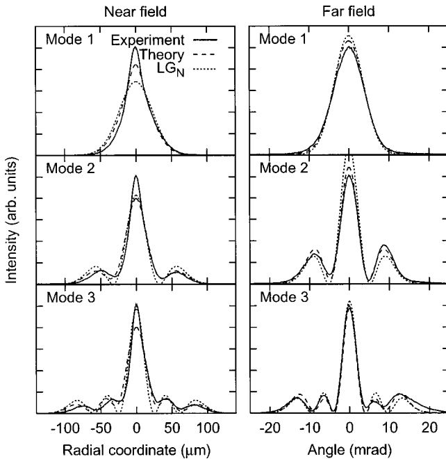
Fig. 6. Left, near-field and, right, far-field mode profiles at reflectivity R_m = 94\% . Three modes are found in the experiment (solid curves). These profiles match the results from the theoretical model (dashed curves) quite well. In contrast, both deviate from the three lowest-order Laguerre–Gaussian TEM modes of the parabolic index guide ( LG_N , dotted curves); the near-field rings are weaker, and the far-field rings are stronger than those of the LG_N modes, and the intensity between rings does not go to zero.
