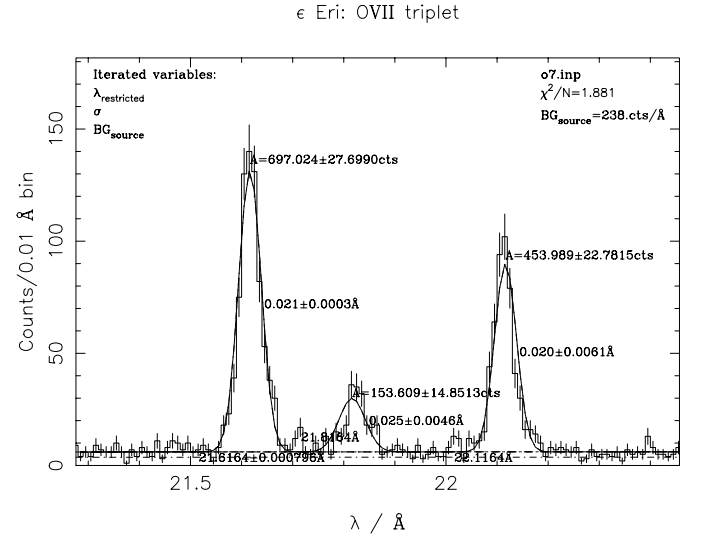
Fig. 5. Measurement of the O VII triplet for \epsilon Eri (105 ksec).
