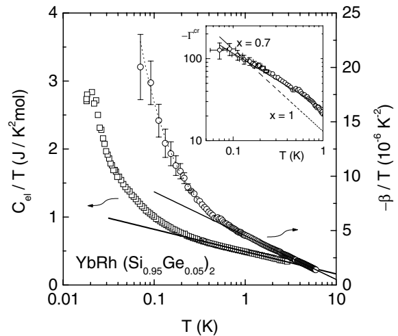
FIG. 4. Electronic specific heat as C_{el}/T (left axis) and volume thermal expansion as -\beta/T (right axis) vs T (on a logarithmic scale) for \text{YbRh}_2(\text{Si}_{0.95}\text{Ge}_{0.05})_2 at B = 0 . The solid lines indicate \log(T_0/T) dependences with T_0 = 30 K and 13 K for C_{el}/T and -\beta/T , respectively. The dotted line represents -\beta/T = a_0 + a_1/T with a_0 = 3.4 \times 10^{-6} \text{ K}^{-2} and a_1 = 1.34 \times 10^{-6} \text{ K}^{-1} . The inset displays the log-log plot of \Gamma^{cr}(T) with \Gamma^{cr} = V_m/\kappa_T \cdot \beta^{cr}/C^{cr} using \kappa_T = 5.3 \times 10^{-12} \text{ Pa}^{-1} [26], \beta^{cr} = \beta(T) + a_0T , and C^{cr} = C_{el}(T) . The solid and dotted lines represent \Gamma^{cr} \propto 1/T^x with x = 0.7 and x = 1 , respectively.
