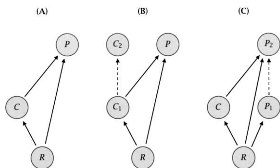
Figure 1: Different cases of IGP and stage structure analyzed in this article. A , Basic intraguild predation. Species P (predator) preys on species C (consumer), and, in addition, P and C compete for a common resource R . B , Structured consumer case. As A but with a second consumer stage ( C 2 ) that is invulnerable to predation. C , Structured predator case. As A but with an initial stage for the predator ( P 1 ) that feeds exclusively on the resource. Solid arrows reflect feeding interactions, and dashed arrows reflect growth transitions.
