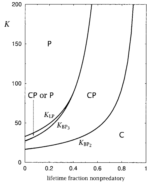
Figure 7: Effect of the relative duration of the nonpredatory stage in the structured predator model on the possible equilibria attained along a productivity gradient. The relative duration, plotted on the abscissa, is given by \mu_p/(\mu_p + m_p) . For explanation, see the text. See table 1 for parameter values.
