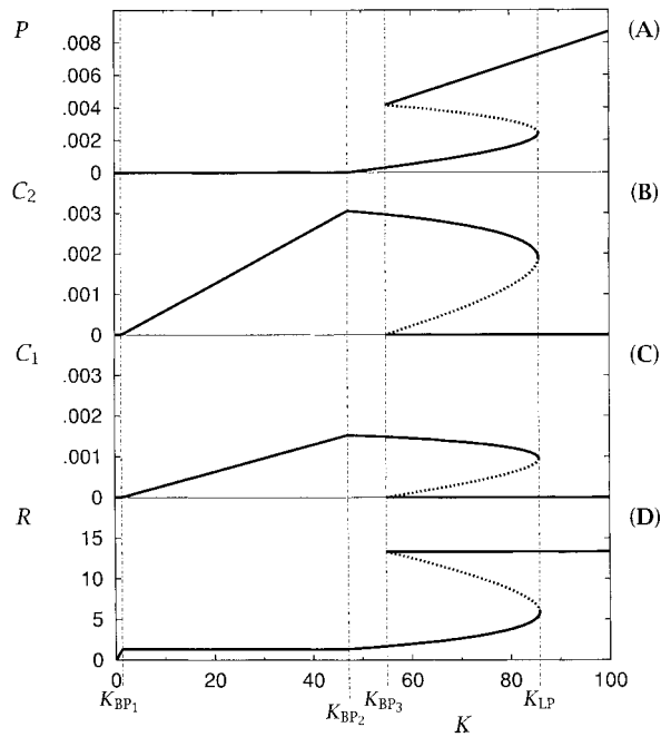
Figure 4: Steady states of the structured consumer model (11)–(14) along a productivity gradient. A , Equilibrium values of the predator population density. B , Equilibrium values of the invulnerable consumer population. C , Equilibrium values of the vulnerable consumer. D , Equilibrium values of the resource. Solid curves , stable equilibria; dotted curves , unstable equilibria. See table 1 for parameter values; m_c = 0.1 \text{ d}^{-1} .
