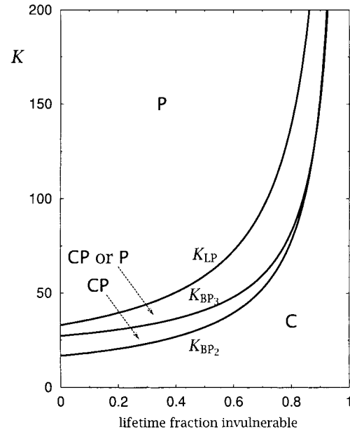
Figure 5: Effect of the relative duration of the invulnerable stage in the structured consumer model on the possible equilibria attained along a productivity gradient. The relative duration, plotted on the abscissa, is given by \mu_c / (\mu_c + m_c) . For explanation, see the text. See table 1 for parameter values.
