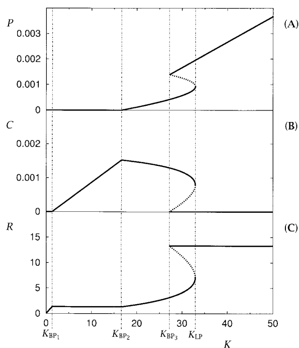
Figure 2: Steady states of the basic IGP model (1)–(3) along a productivity gradient. A , Equilibrium values of the predator population density. B , Equilibrium values of the consumer population. C , Equilibrium values of the resource. Solid curves denote stable equilibria, dotted curves unstable ones. Parameter values are listed in table 1.
