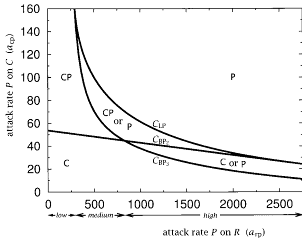
Figure 3: Effect of the attack rates a_{rp} and a_{cp} on the existence of possible equilibria of the basic IGP model (1)–(3). Curve C_{LP} corresponds to K_{LP} , curve C_{BP_2} to K_{BP_2} , and curve C_{BP_3} to K_{BP_3} (cf. fig. 2). For every region bounded by these curves, the stable steady states are indicated: P denotes the predator equilibrium, C the consumer equilibrium, and CP the consumer-predator equilibrium. The variable K = 32.94 \text{ ind}_r \times L^{-1} , and the other parameters have values as listed in table 1.
