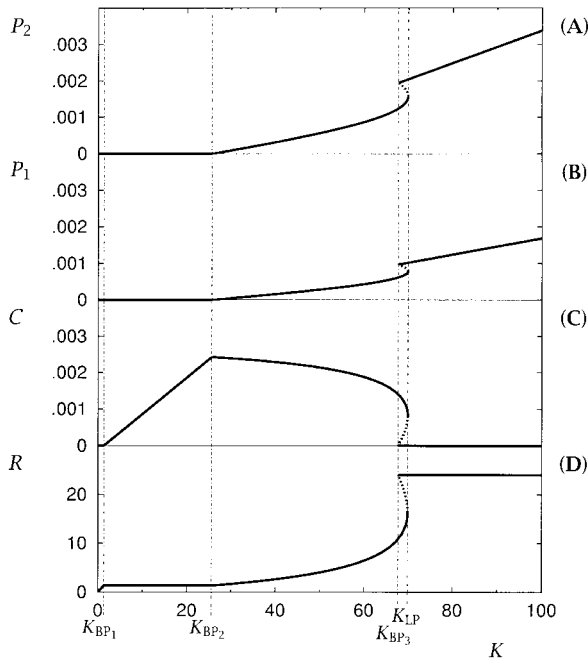
Figure 6: Steady states of the structured predator model (16)–(19) along a productivity gradient. A, Equilibrium values of the second-stage predator population density. B, Equilibrium values of the initial-stage predator population. C, Equilibrium values of the consumer. D, Equilibrium values of the resource. Solid curves, stable equilibria; dotted curves, unstable equilibria. See table 1 for parameter values; m_p = 0.1 \text{ d}^{-1} .
