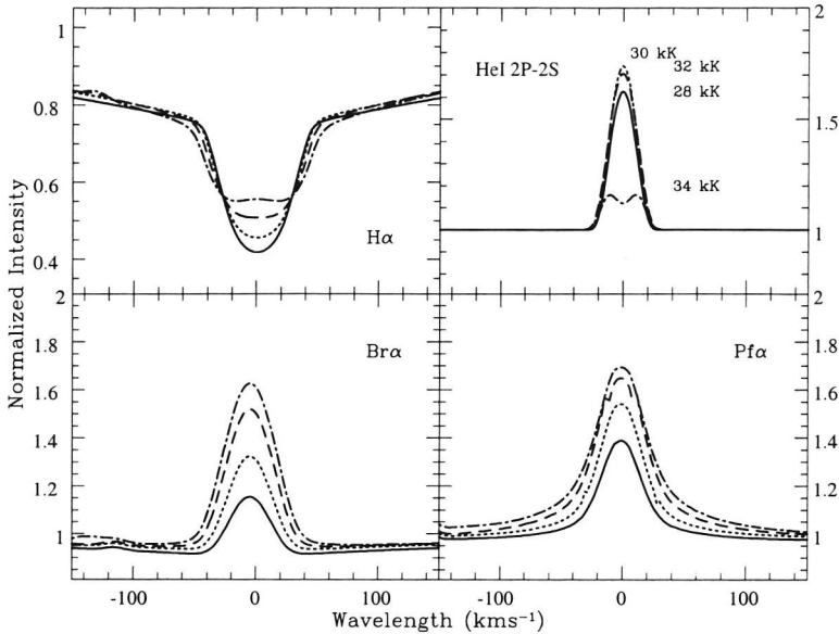
Figure 4.11. Effective temperature dependence of H\alpha , \text{He I } \lambda 2.058 , \text{Br}\alpha , and \text{Pf}\alpha , predicted using H&He models (as in Fig. 4.10). For \text{He I } \lambda 2.058 the corresponding T_{\text{eff}} is given at the level of maximum line flux.
