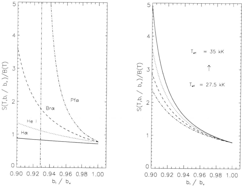
Figure 4.5. The left panel shows the dependence of the line over continuum source function ratio, S_{l,\nu}/B_\nu , as a function of b_l/b_u for H \alpha , He I \lambda 2.058, Br \alpha , and Pf \alpha . Characteristic temperatures are T_e^* = 32.5 kK and T_e = 0.8 T_e^* . The right panel shows the dependence as a function of stellar effective temperature for Br \alpha . Four values are indicated, T_{\text{eff}} = 27.5, 30, 32.5 and 35 kK.
