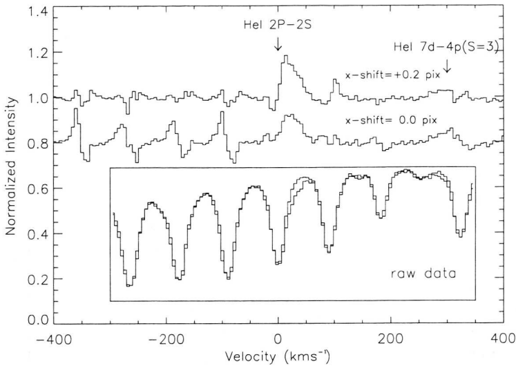
Figure 4.3. The He I 2.058 \mu\text{m} spectrum as observed with UKIRT. The top spectrum as reduced with a slight shift of 0.2 pixel ( 1.1 \text{ km s}^{-1} ) for the ratio star, HR6366. The bottom spectrum as reduced without shifting the ratio star. Also the “raw” spectra of \tau Sco and HR6366 are given to illustrate the strong telluric lines present.
