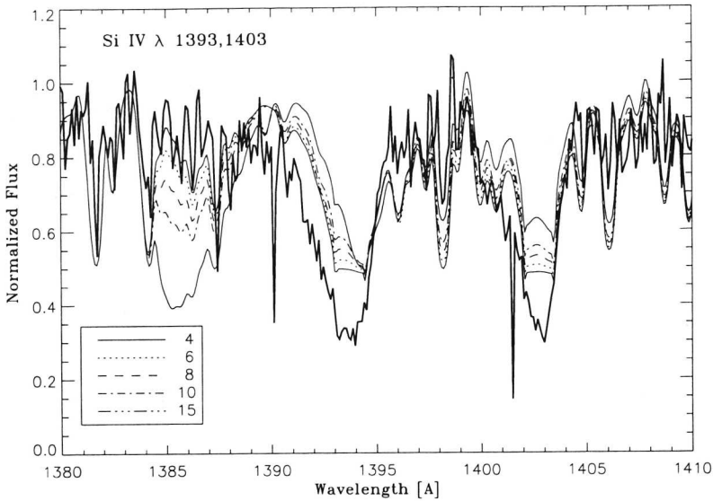
Figure 4.7. The observed Si IV line profile of \tau Sco and the synthetic spectra as derived with the ISA-WIND code for five different mass-loss rates, given in the legend in units of 10^{-9} M_{\odot} \text{yr}^{-1} . Increasing \dot{M} yields progressively more absorption at large blueshifts, which can be used to derive an upper limit of the mass-loss rate of \sim 6 \cdot 10^{-9} M_{\odot} \text{yr}^{-1} .
