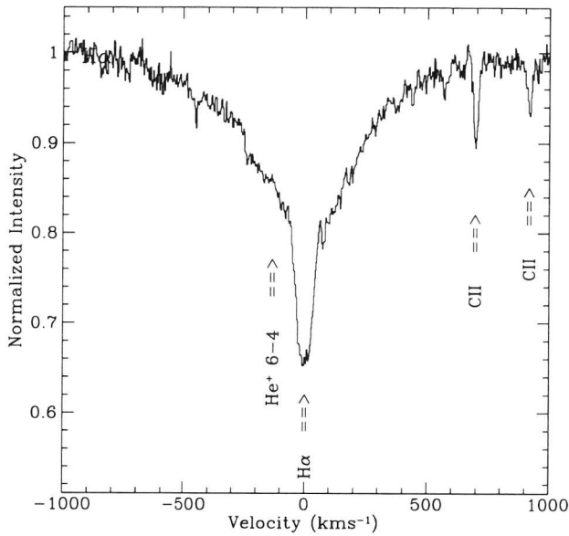
Figure 4.1. H \alpha observed in 1996 May 2nd with INT during commissioning of the MUSICOS instrument.
