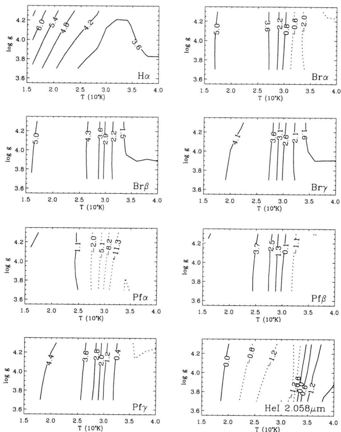
Figure 4.8. Predicted T_{\text{eff}} - \log g contour plots for eight line profiles. The contours represent the equivalent width (in \text{\AA} ) of the line profiles between -/+ 300 \text{ km s}^{-1} , except for \text{H}\alpha where we used an interval between -/+ 1000 \text{ km s}^{-1} . Solid (dashed) lines indicate net absorption (emission).
