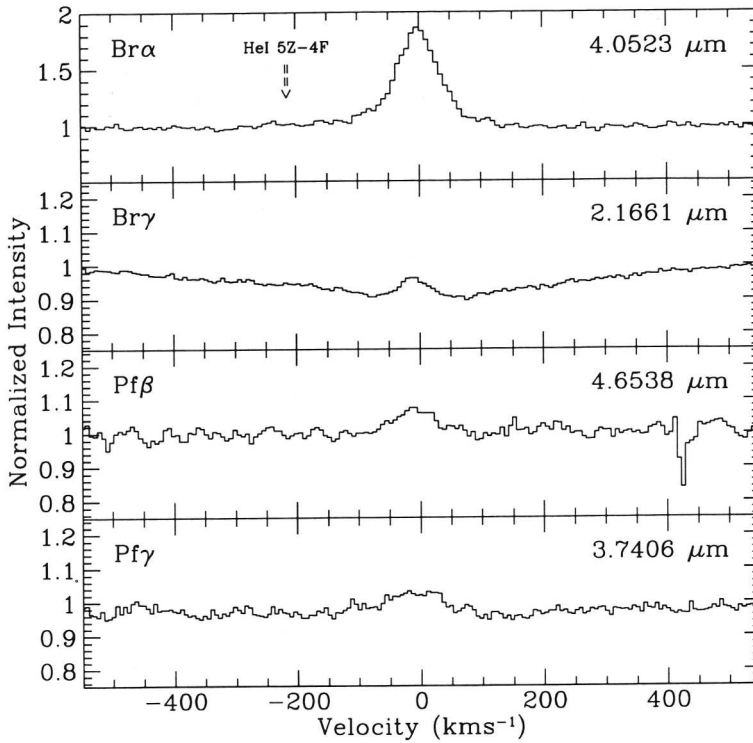
Figure 4.2. UKIRT observations of hydrogen emission profiles in \tau Sco.
