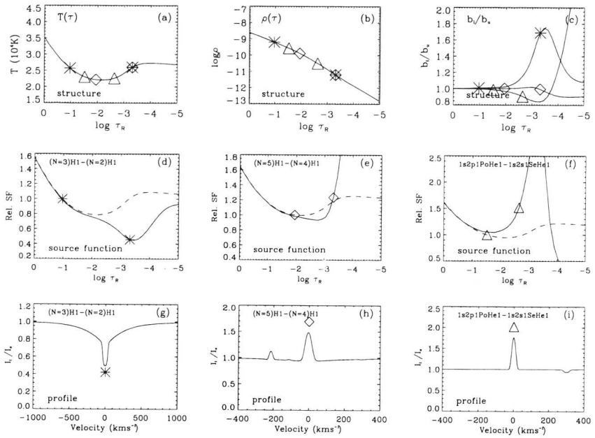
Figure 4.6. An overview of the atmospheric structure and of the line and continuum source functions for three lines: H \alpha , Pf \alpha and He I \lambda 2.058. The bottom three panels show respective predicted line profiles. Information about different lines is indicated with different symbols. Data are for a TLUSTY model atmosphere with T_{\text{eff}} = 31.4 kK and \log g = 4.24 . The top panels show the run of temperature, density and b_l/b_u with Rosseland optical depth. Marked are the positions where line core and continuum reach optical depth \tau = 2/3 . The non-LTE line (solid line) and continuum (dashed line) source functions given in the middle three panels are normalized to the continuum source function value at continuum \tau = 2/3 .
