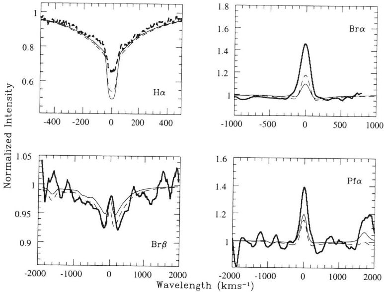
Figure 4.14. Comparison of fully line blanketed (dashed line) and H&He model (solid line) with UKIRT observations (as in Fig. 4.13). The line blanketed model gives an improved fit to \text{Br}\alpha and \text{Br}\gamma , but yields a poorer fit to \text{Pf}\beta .
