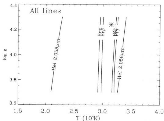
Figure 4.9. T_{\text{eff}} - \log g diagram in which for each line are plotted the contours where the predicted equivalent width matches the observed one. Predictions are based on H&He models. The *-symbol indicates the basic parameters of \tau Sco as determined by Kilian (1992), i.e. T_{\text{eff}} = 31.4 \pm 0.3 kK and \log g = 4.24 \pm 0.03 . For He I \lambda 2.058 the EW matches two contours as the predicted EW shows a maximum at \sim 25 -30 kK (see Fig. 4.8). The observed EW of H \alpha , Br \alpha , and Pf \alpha fall outside the range of this plot (see text).
