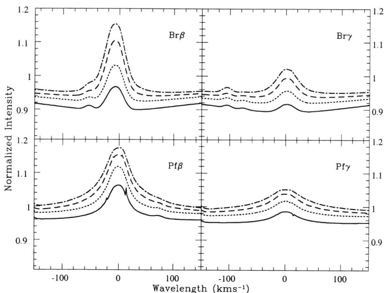
Figure 4.10. Profiles of four IR lines ( \text{Br}\beta , \text{Br}\gamma , \text{Pf}\beta , \text{Pf}\gamma ) as predicted using H&He models for four values for T_{\text{eff}} : 28 kK (solid), 30 kK (dotted), 32 kK (short dashed) and 34 kK (long dashed). Gravity is kept fixed at \log g = 4.3 .
