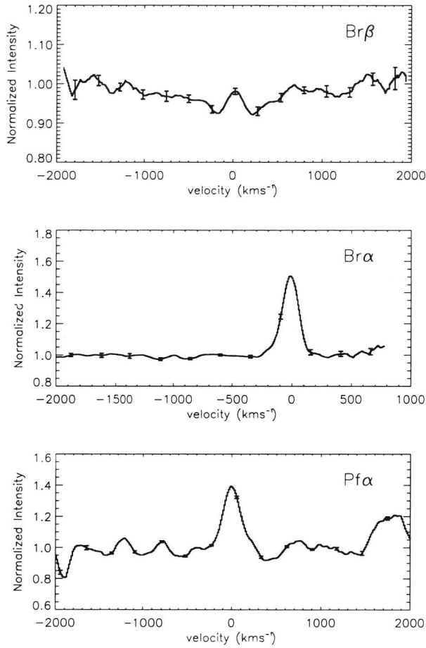
Figure 4.4. ISO observations of IR hydrogen profiles in \tau Sco.
