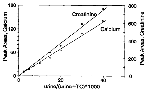
Fig. 3. Peak area as function of dilution factor for urinary calcium and creatinine. Other conditions as in Fig. 2.
