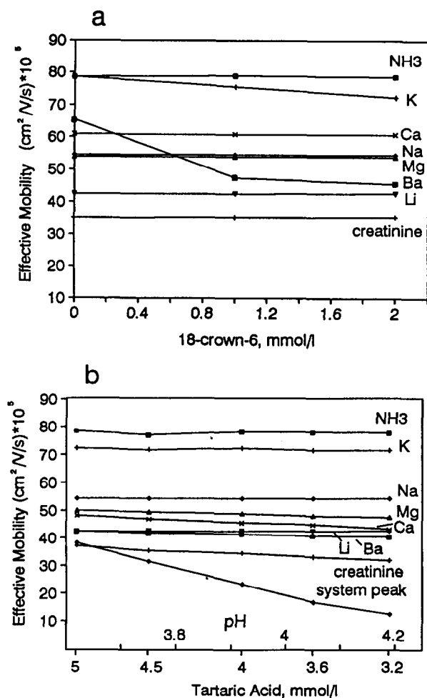
Fig. 1. The influence of 18-crown-6 (a) and tartaric acid (b) on mobilities of cations. BGEs are BGE II (a) and BGE I (b) but with varying amounts of 18-crown-6 and tartaric acid, respectively. All other details are as described in Table 1.
