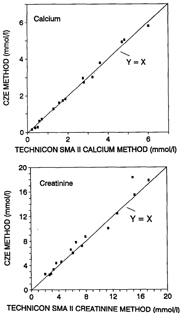
Fig. 4. Correlations between CZE method and Technicon SMA II methods. The regression line parameters obtained from this study are (calcium) y = -0.03 + 1.013x , r^2 = 0.9960 , n = 16 ; (creatinine) y = -0.03 + 1.052x , r^2 = 0.9671 , n = 17 .
