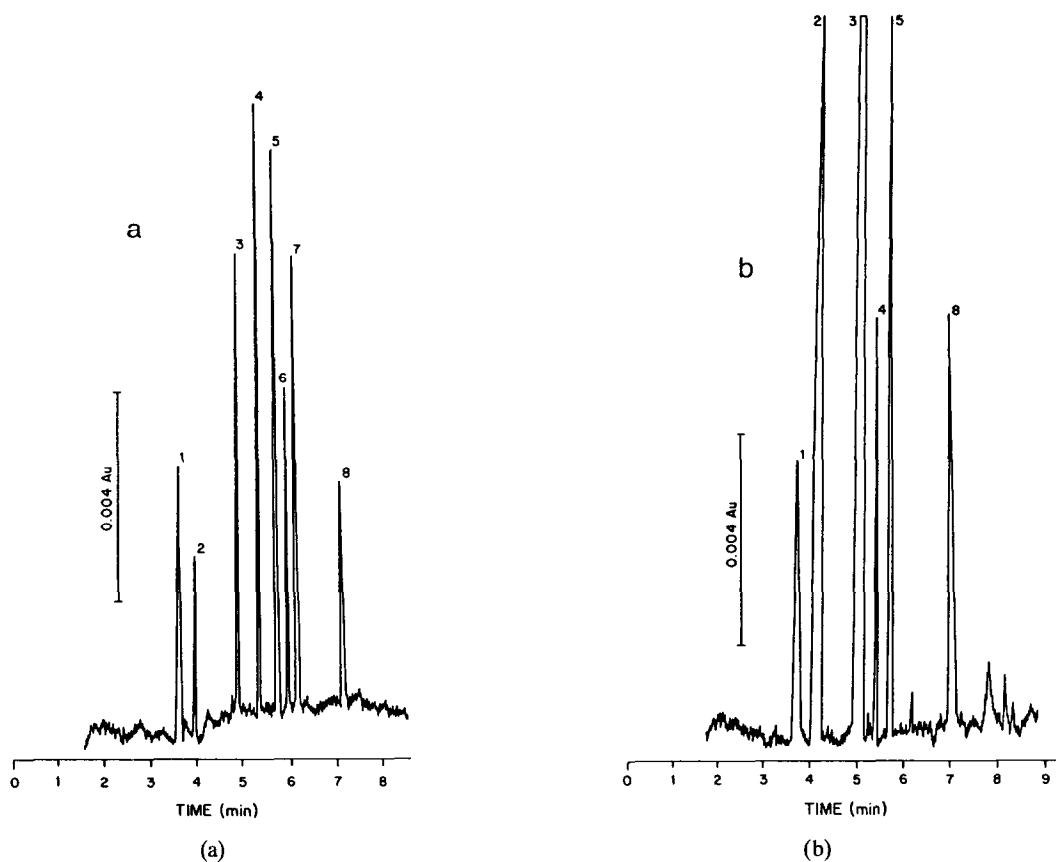
Fig. 2. Electropherograms of standard solution (a), urine samples from a normal person (b), a patient with complicated urinary composition (c), and a patient with extremely low urinary calcium level (d). Electrophoresis was performed with BGE I. The concentration of each cation in the standard solution is 0.1 mmol/l. Dilution factors and urinary levels (mmol/l) of calcium and creatinine for each urine specimen are 1:50, 4.94, 6.06 (b); 1:50, 3.03, 6.56 (c); 1:25, 0.29, 17.85 (d). The numbers of the peaks are according to Table 1. Conditions are as described in Experimental.
