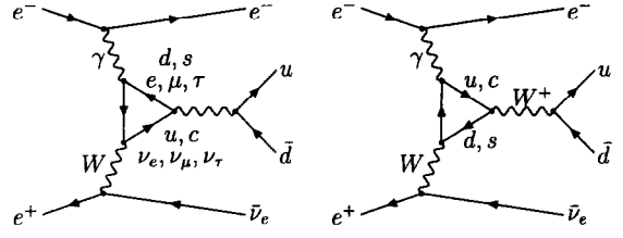
Fig. 2. The extra fermionic diagrams needed to cancel the gauge-breaking terms.
