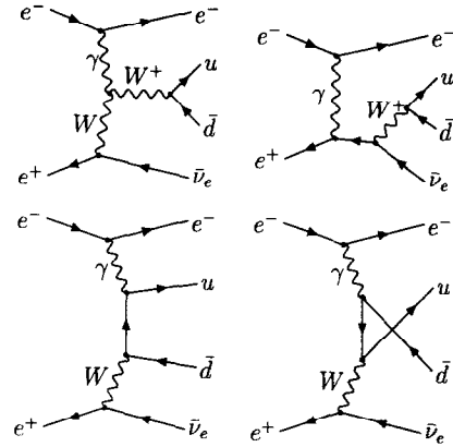
Fig. 1. The four diagrams of the process e^-e^+ \rightarrow e^-\bar{\nu}_e u\bar{d} which are considered here.
