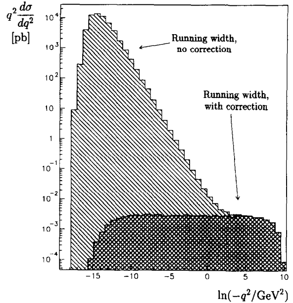
Fig. 3. The effect of gauge-breaking terms in e^-e^+ \rightarrow e^-\bar{\nu}_e u\bar{d} as a function of the virtuality of the photon.
