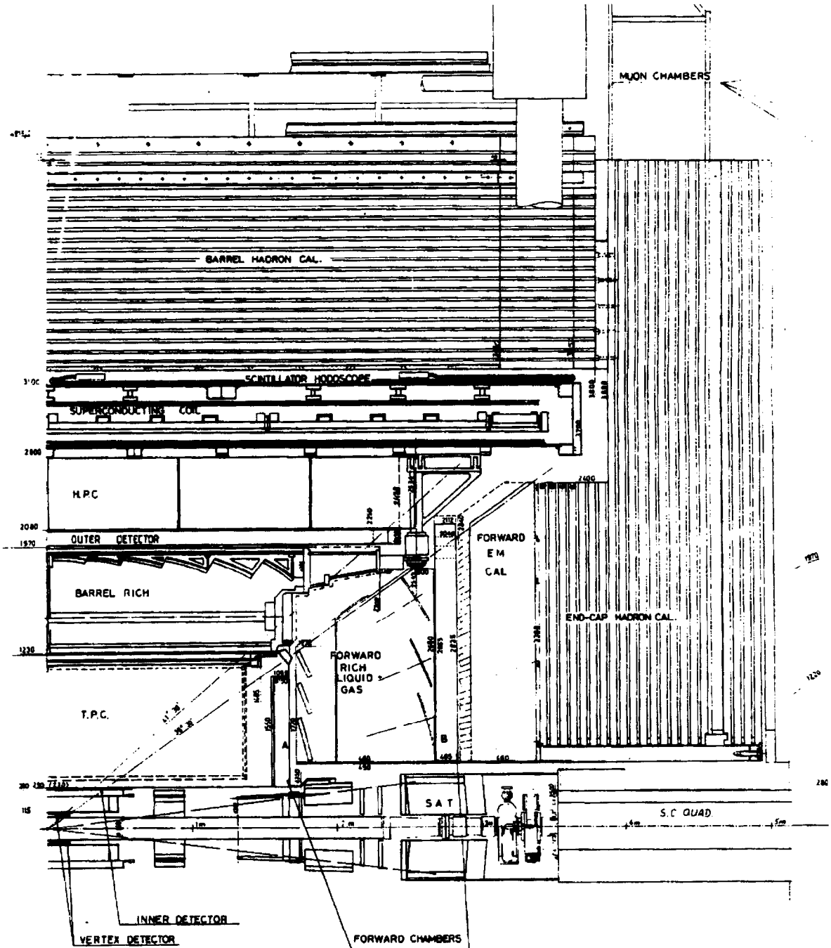
Fig. 1. Cross section along the beampipe of a quarter of the DELPHI detector. The Forward and Barrel RICH are sandwiched between the different tracking detectors: Time Projection Chamber (TPC), Outer Detector (OD), Forward Chambers A and B (FCA, FCB).
