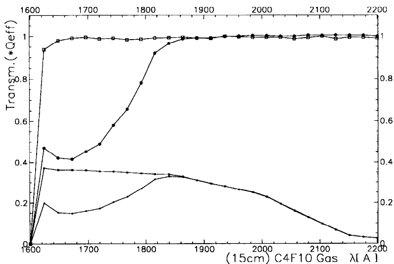
Fig. 2. UV transmission vs wavelength (in Å) of the Forward RICH C_4F_{10} gas radiator. ● = before start of 1994 physics, running, \int_{1600}^{2200} (Tr \times Q_{eff}) = 117 Å. □ = during normal operation, \int_{1600}^{2200} (Tr \times Q_{eff}) = 148 Å. The difference in transmission can be explained by a 450 ppm water contamination.
