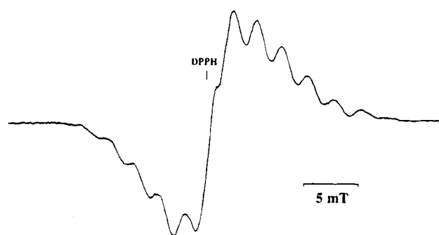
Figure 4. ESR spectrum of [\text{MnRe/BPYM/Re}]^{\cdot-} in THF at 293 K.
