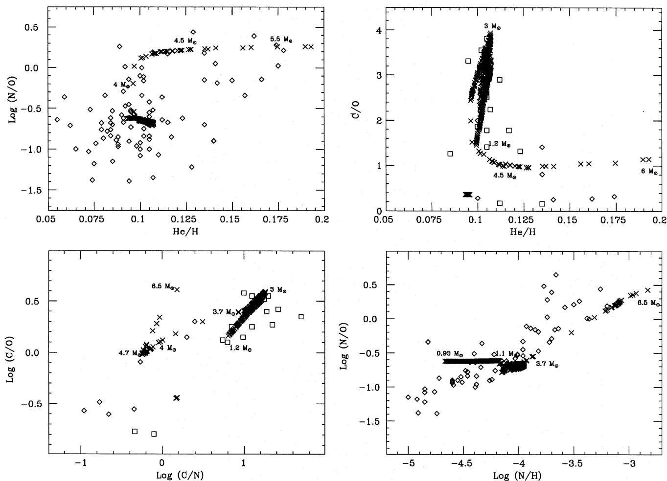
Fig. 1. Observed and predicted abundance ratios of planetary nebulae in the LMC for the standard model. Model results are plotted as crosses and some initial masses are indicated. In the C/O – \text{He}/H and C/O – C/N diagram the observed type I PNe (defined as having N/O > 0.5 ) are indicated by diamonds, the other observed PNe by squares. The density of points of the model stars with increasing initial mass reflects the initial mass function and the star formation rate history
