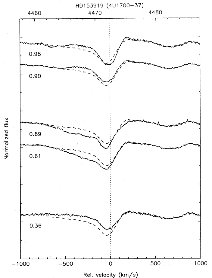
Fig. 6. As Fig. 1; The He I line of HD153919 at 4471 Å. Around \phi = 0.6 the blue-shifted absorption gets much stronger over a wide velocity range, similar to the H \beta line displayed in Fig. 4
