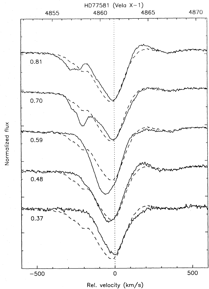
Fig. 1. Normalized H \beta profiles of HD77581 (Vela X-1). The spectra have been shifted vertically according to their orbital phase, indicated at the left side of each spectrum. The tickmarks on the vertical scale are placed at 10% intervals. The dashed line represents the average spectrum. Note, however, that the spectra at \phi = 0.6 and \phi = 0.7 are not sequential: we started the observations at \phi = 0.7
