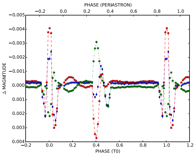
Figure 5. Shown is a comparison of the residuals of each fit: LM-MM (red), LM-HM (blue), and MM-HM (green). Each fit has a standard deviation of around 2.5 mmas. They are very nearly identical to each other in all places except in the eclipses.
