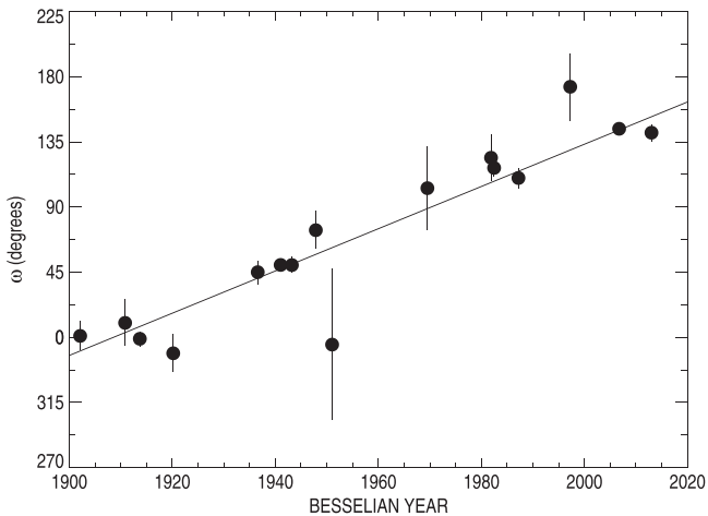
Figure 6. Apsidal motion of \delta Ori. A weighted linear fit to the published values (Harvey et al. 1987, H02, M10) yields a measurement of \dot{\omega} = (1.45 \pm 0.04) \text{ yr}^{-1} .
