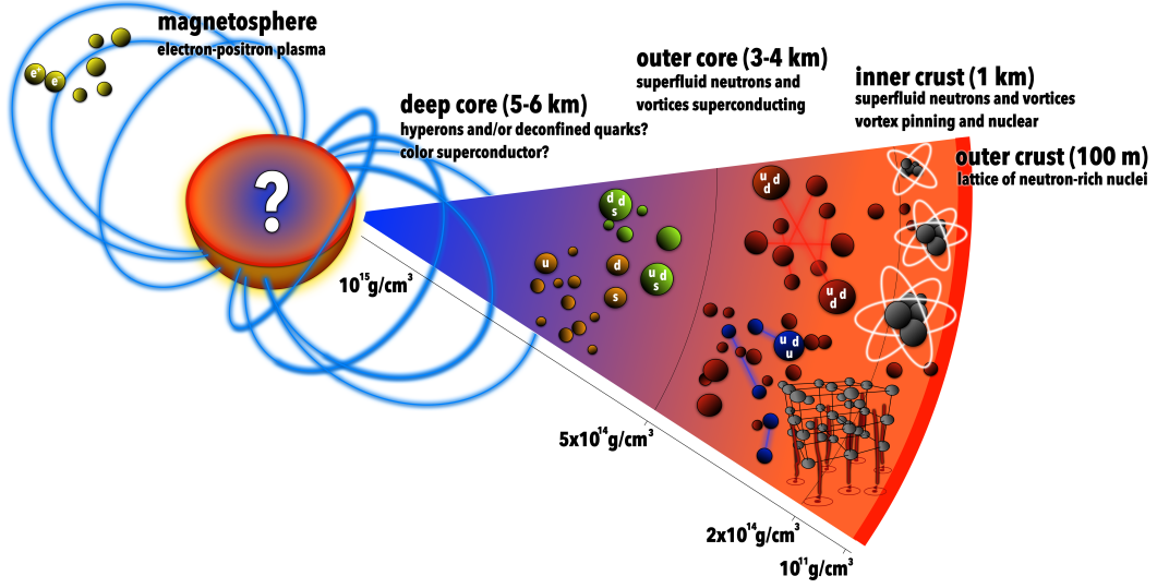
Figure 1: Schematic structure of a NS. The outer layer is a solid ionic crust supported by electron degeneracy pressure. Neutrons begin to leak out of nuclei at densities \sim 4 \times 10^{11} \text{ g/cm}^3 (the neutron drip line, which separates inner and outer crust), where neutron degeneracy also starts to play a role. At densities \sim 2 \times 10^{14} \text{ g/cm}^3 , the crust-core boundary, nuclei dissolve completely. In the core, densities may reach up to ten times the nuclear saturation density \rho_{\text{sat}} = 2.8 \times 10^{14} \text{ g/cm}^3 (the density in normal atomic nuclei).
