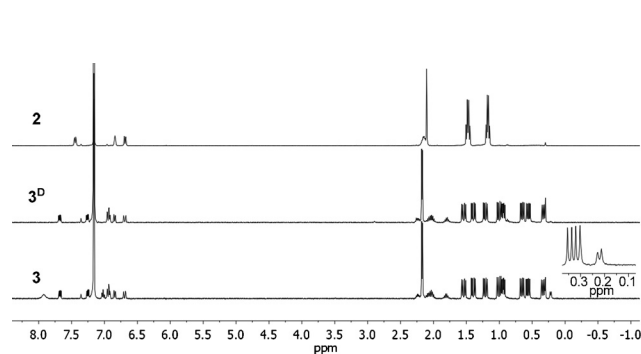
Figure 2. 1 H NMR spectra before (top), after irradiation of 2 in C 6 D 6 (middle), and after irradiation in C 6 H 6 (bottom). The insert is showing an additional (-NH) doublet at 0.22 ppm for the irradiation in C 6 H 6 .
