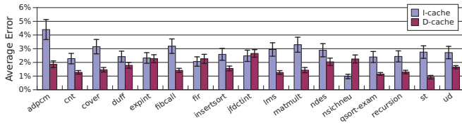
Fig. 3. Average missrate prediction error (over the complete range of cache configurations). The error bars show the standard deviation.
