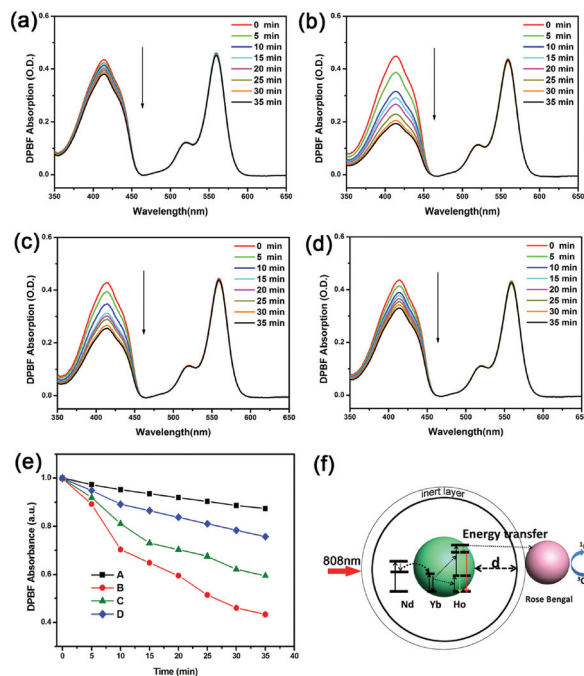
Fig. 4 Absorption spectra measured every 5 minutes of DPBF ( 10\ \mu\text{L} , 8\ \text{mM} ) incubated with \text{NaYF}_4\text{:Yb/Ho}(8/1\%)\text{@NaYF}_4\text{:Nd}(20\%)\text{@NaYF}_4 with different \text{NaYF}_4\text{:Nd}(20\%) active-shell thicknesses under irradiation at 808\ \text{nm} : (a) sample A ( 0.4\ \text{nm} ); (b) sample B ( 1.6\ \text{nm} ); (c) sample C ( 2.5\ \text{nm} ); (d) sample D ( 4.2\ \text{nm} ). (e) Absorbance at 410\ \text{nm} of DPBF in ethanol solutions of A–D as a function of irradiation time. (f) Illustrated diagram showing the different \text{NaYF}_4\text{:Nd}(20\%) active-layer thicknesses of the nanoparticles for the production of ^1\text{O}_2 .
