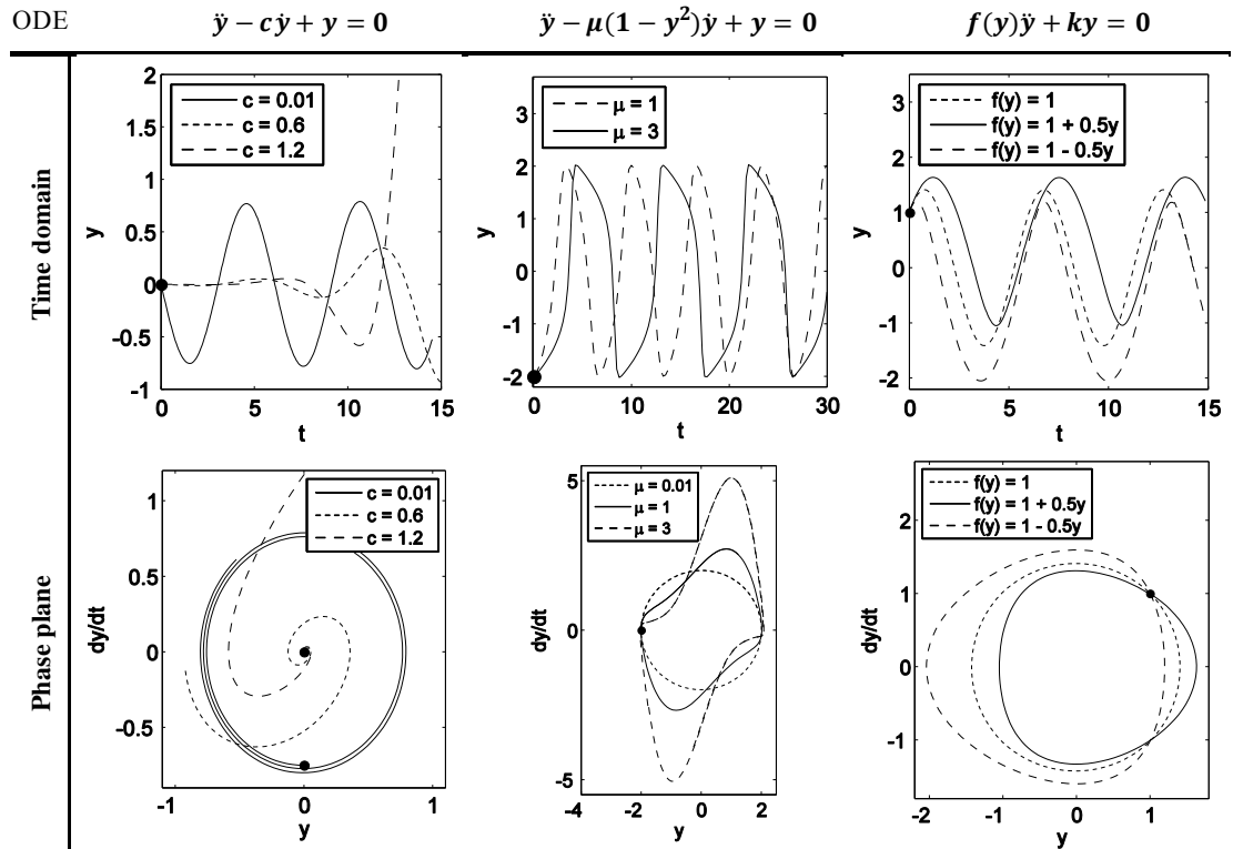
Figure 1: Vibration examples shown in time domain (upper row) and in phase plane (lower row). Left column: constant negative damping; middle column: non-linear damping by Van der Pol oscillator; right column: non-linear mass term. The corresponding ODE equations are written on top; y is the vertical displacement of the mass. The initial states are indicated by thick dots.
