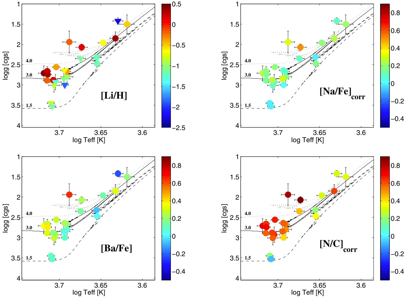
Fig. 13. Variations of some key abundance ratios across the \log T_{\text{eff}} - \log g plane. For the NLTE lithium abundances, the downward-pointing triangles denote upper limits. The predictions at solar metallicity of evolutionary models for masses of 1.5, 3, and 4 M_{\odot} are overplotted for illustrative purposes. Same tracks as in Fig. 1, except that the evolutionary phase, is not colour coded.
