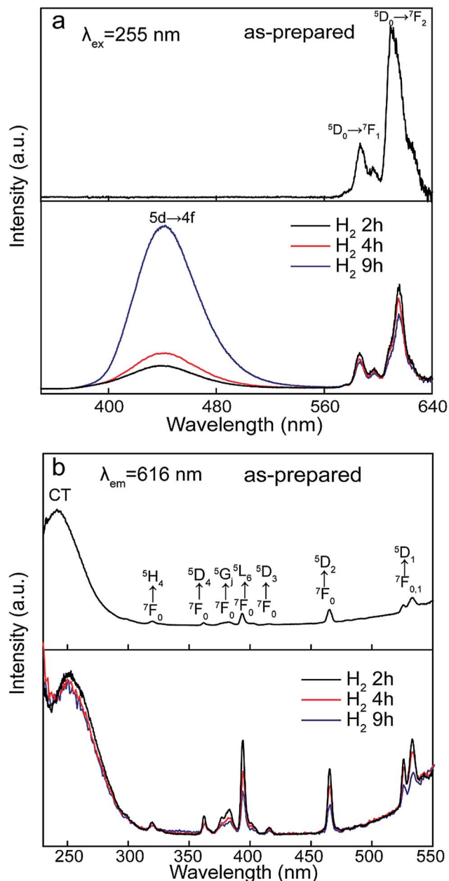
Fig. 3 (a) Emission ( \lambda_{\text{ex}} = 255 \text{ nm} ) and (b) excitation ( \lambda_{\text{em}} = 616 \text{ nm} ) spectra of the as-prepared and the annealed samples.
