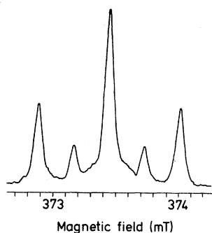
FIG. 7. Lineshape of spectrum NL21 in a sample with 89% ^{57}\text{Fe} . Spectrum for orientation da with \vec{B} 0.5^\circ out of the [100] direction in the (0\bar{1}1) plane, \nu = 22.8722 GHz, and a sample temperature of 1.4 K.
