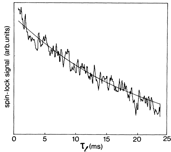
FIG. 5. Optically detected spin-locking decay at 2.319 GHz and 1.4 K for the F_2^{2+} center in MgO in zero field. Drawn line is monoexponential fit with \tau_{decay} = 20 ms.
