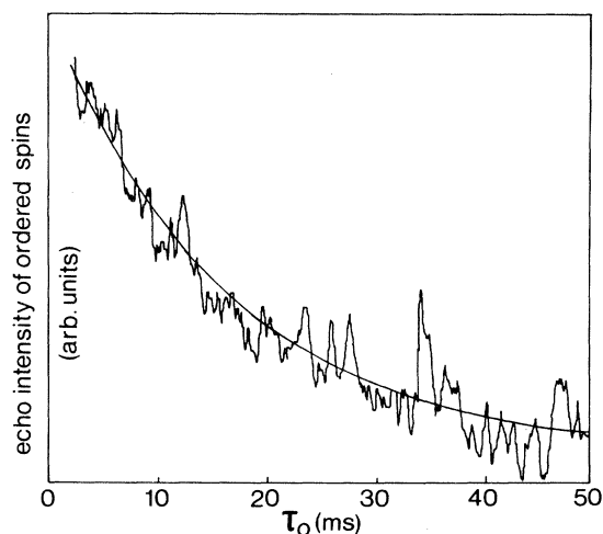
FIG. 6. Optically detected spin-echo decay in the ordered ^3B_{1u} state of the MgO F_2^{2+} center as monitored for the |D\rangle - |E\rangle transition at zero field, T = 1.4 K. Drawn line is monoexponential fit with \tau_{decay} = 16 ms.
