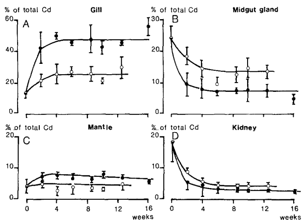
Fig. 2. Distribution of Cd (as % of total body burden) vs exposure time in four organs of A. cygnea , exposed to 25 ppb Cd (—●—) or to 25 ppb Cd plus 2.5 ppm Zn (—○—). Mean \pm SD of four animals
