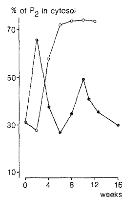
Fig. 5. Percentage of Cd bound to P_2 in the gill cytosolic fraction during exposure to 25 ppb Cd (—●—), or 25 ppb Cd + 2.5 ppm Zn (—○—). Pooled organs of four animals
