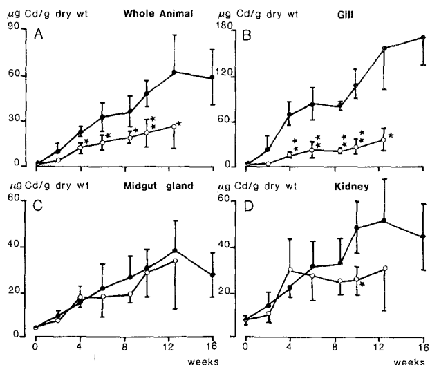
Fig. 1. Cd concentrations vs exposure time in whole body and some organs of A. cygnea , exposed to 25 ppb Cd (—●—) or 25 ppb Cd + 2.5 ppm Zn (—○—). Mean \pm SD of four animals; significant differences between Cd and Cd plus Zn groups at each exposure time are denoted by * ( p < 0.05 ) or ** ( p < 0.01 )
