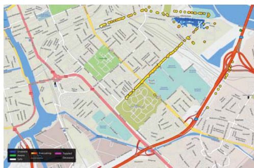
Simulation results in the UrbanFlood decision support system: dike breach, flood dynamics, and evacuation modeling for Science Park, Amsterdam.
