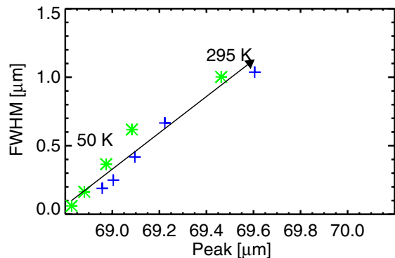
Fig. 3. Effect of the shape model used for the forsterite grains on the peak position and FWHM. Shown as blue crosses is the distribution of hollow spheres (Min et al. 2003) while green asterisks stand for Mie scattering on spherical grains. Both examples are based on the data from Suto et al. (2006) and cover the temperature range from 50 to 295 K. The grain size is 0.1 \mu\text{m} and the black arrow indicates the temperature dependency.
