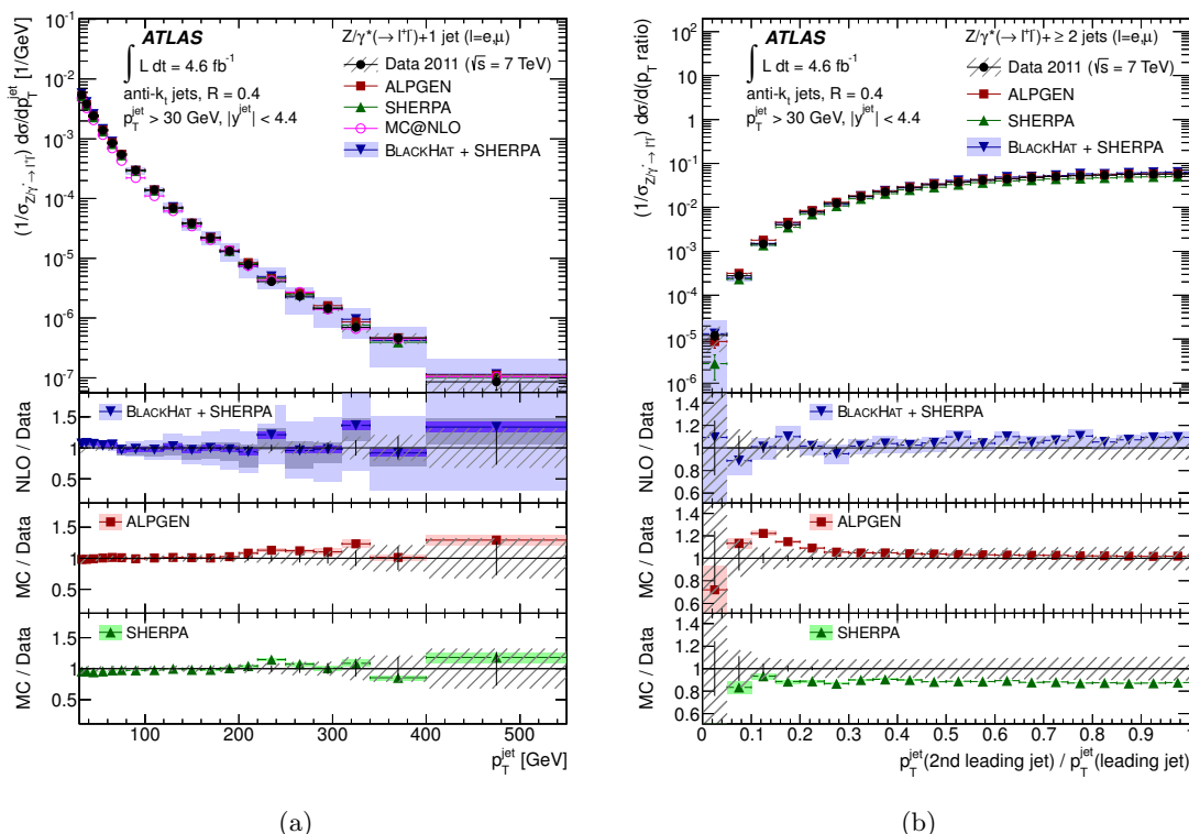
Figure 7. (a) Measured cross section for Z(\rightarrow\ell\ell)+ jets as a function of the jet transverse momentum, p_T^{\text{jet}} , for events with exactly one jet with p_T^{\text{jet}} > 30 GeV and |y^{\text{jet}}| < 4.4 in the final state and (b) as a function of the ratio of p_T^{\text{jet}} of the second leading jet to p_T^{\text{jet}} of the leading jet for events with at least two jets. The cross sections are normalized to the inclusive Z(\rightarrow\ell\ell) cross section. The other details are as in figure 3.
