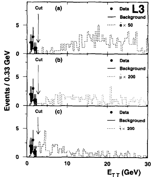
Fig. 1. In (a) we show the distribution for data, expected background and the expected electron signal when only the cut on the variable E_{TT} corresponding to the tau-tau selection is released in the final selection. In (b) we show the same distribution for smuons and in (c) for staus. The signal distributions, which are shown, are the ones obtained for M_{\text{slepton}} = 60 GeV and M_{\tilde{\chi}_1^0} = 23 GeV with the following values of the supersymmetric parameters: M = 40 GeV, \mu = -200 GeV, \tan \beta = 1.5 , m_0 = 50 GeV and A = 0 , for which the expected cross section for selectron is 0.8 pb and 0.4 pb at respectively 136 GeV and 130 GeV of centre of mass energy, while for smuons and staus is 0.14 pb and 0.08 pb at the same centre of mass energies as before.
