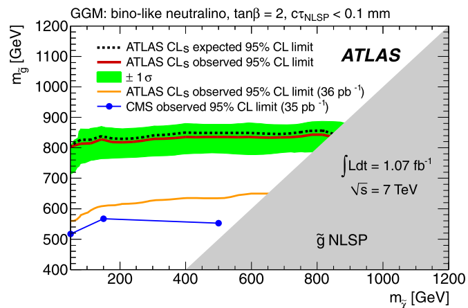
Fig. 4. Expected and observed 95% CL lower limits on the gluino mass as a function of the neutralino mass in the GGM model with a bino-like lightest neutralino NLSP (the grey area indicates the region where the NLSP is the gluino, which is not considered here). The other sparticle masses are fixed to \sim 1.5 TeV. Further model parameters are \tan\beta = 2 and c\tau_{\text{NLSP}} < 0.1 mm. The previous ATLAS [1] and CMS [52] limits are also shown.
